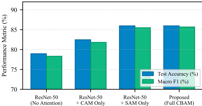
(a) Attention Component Ablation (374 Cohort)
