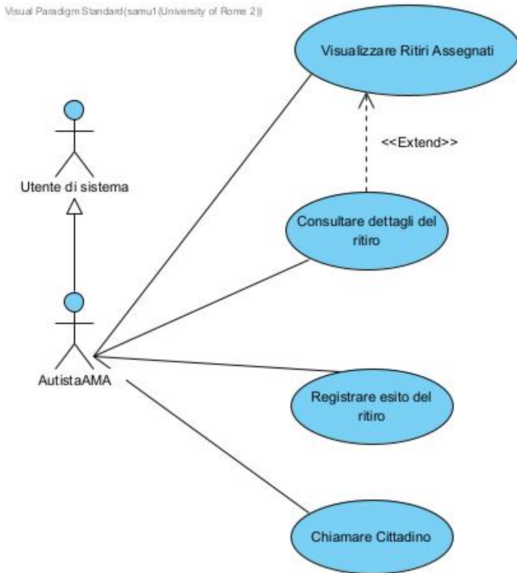
Figura 3: Use Case Diagram — Autista AMA
