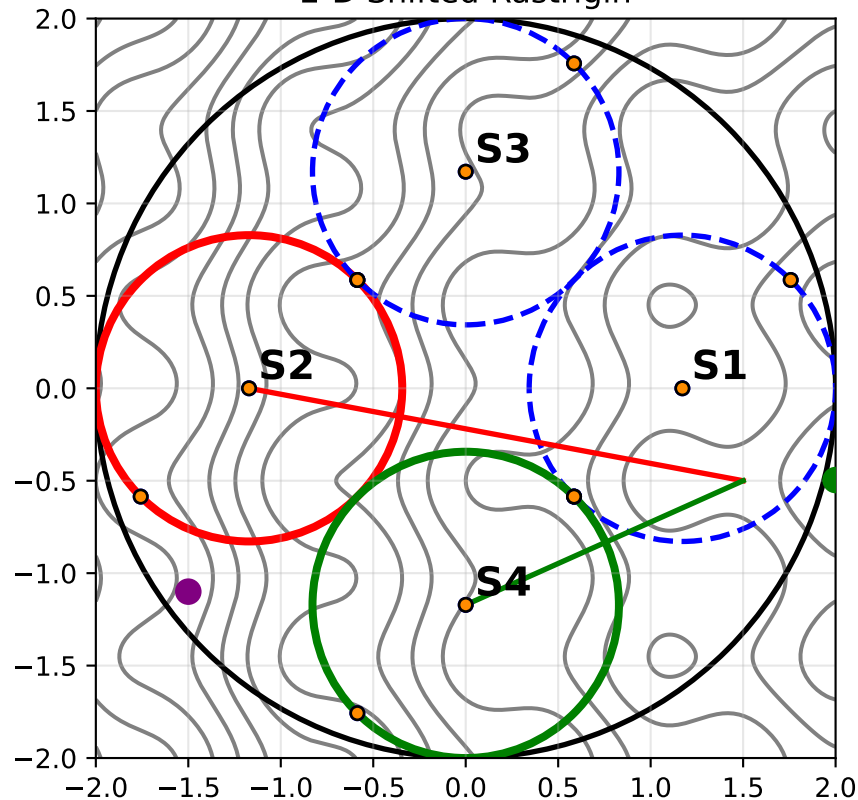
2-D Shifted Rastrigin
