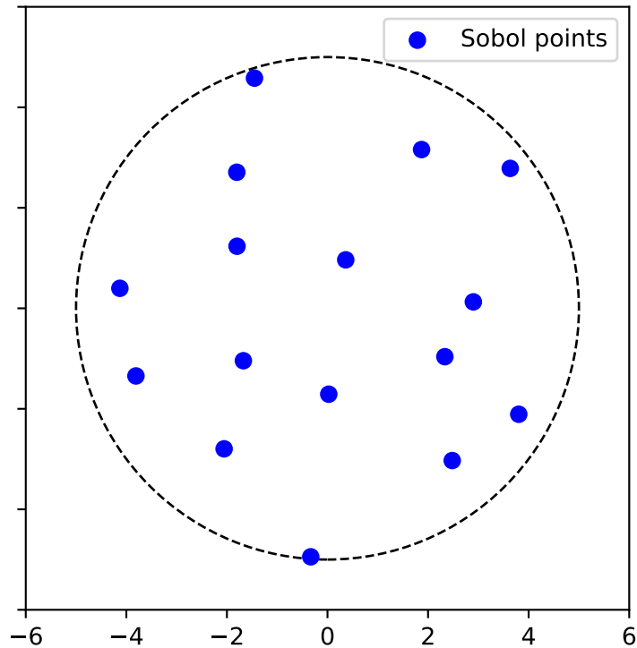
FDA-AS Sobol sampling (n = 16)
