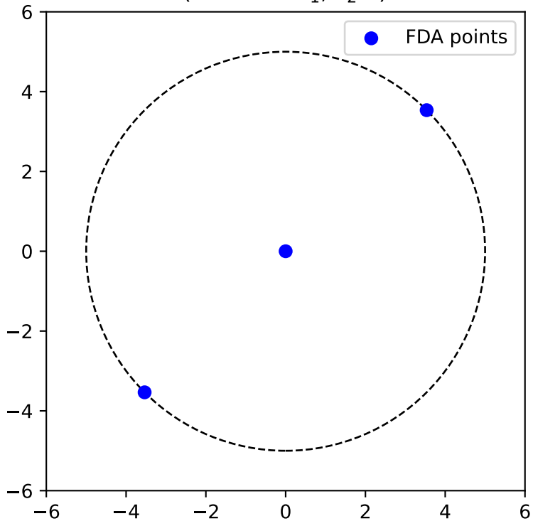
Original FDA sampling (center + s_1, s_2 a)
