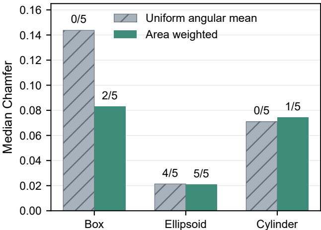
Area-weighting ablation (labels: successes)
