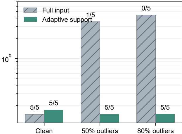
Density-support ablation (labels: successes)
