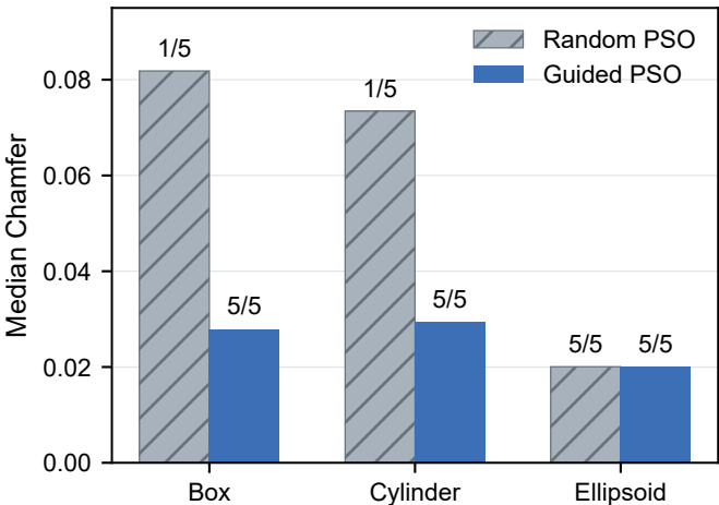
Initialization ablation (labels: successes)
