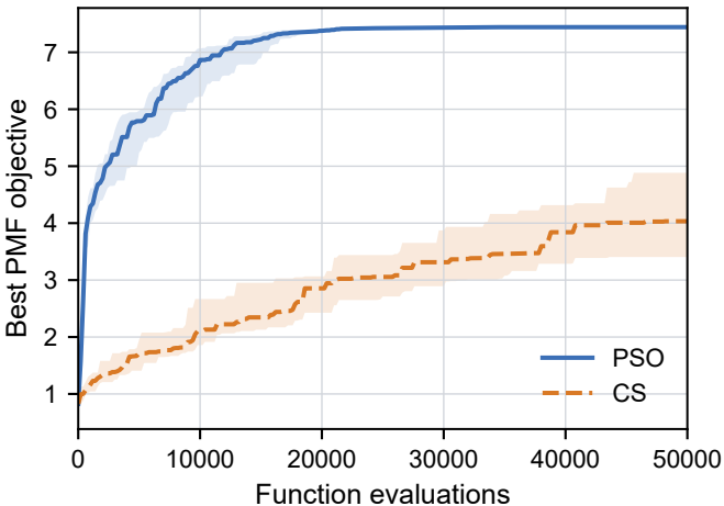
Clean partial-cylinder convergence
