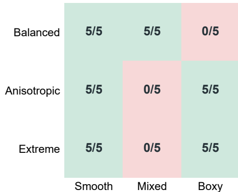
(b) Guided-PSO successes
