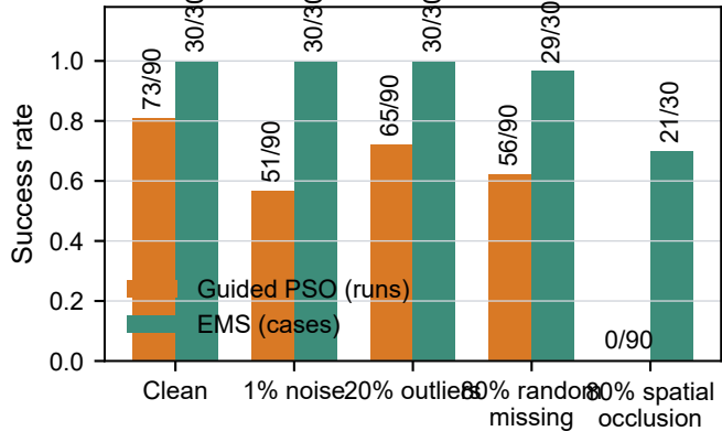
(b) Thresholded recovery
