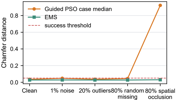
(a) Accuracy across corruption types
