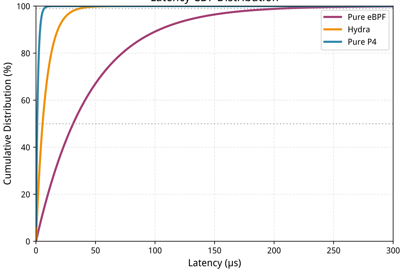
Latency CDF Distribution
