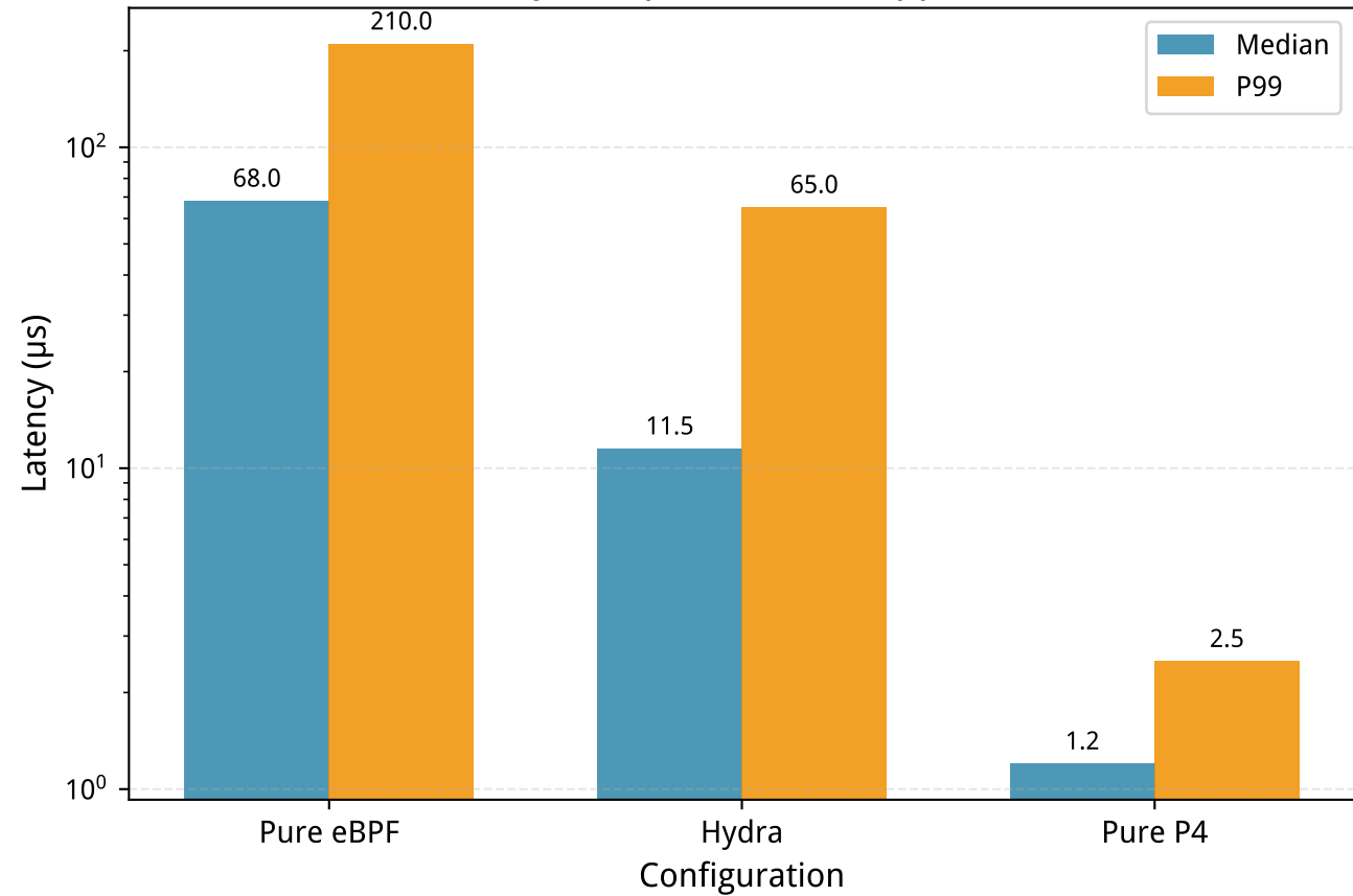
Latency Comparison (100 Kpps Load)
