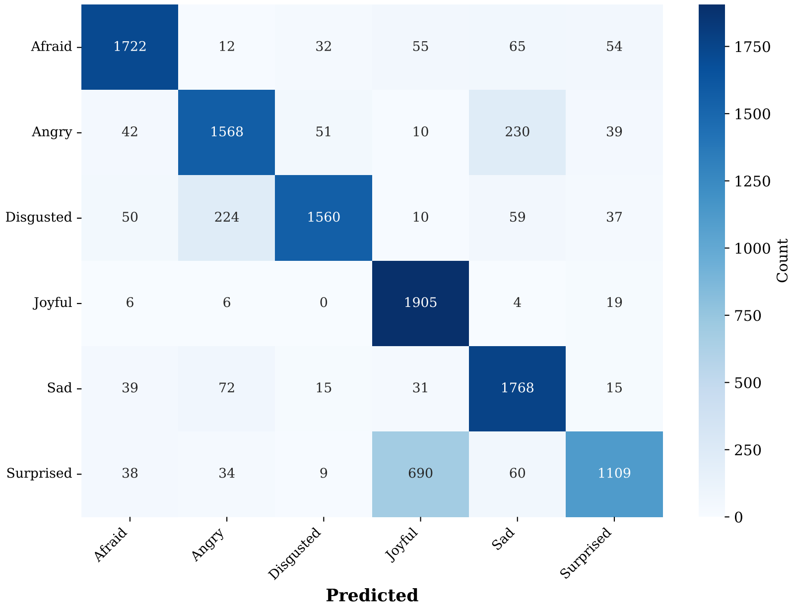
Baseline Confusion Matrix (6-Emotion)
