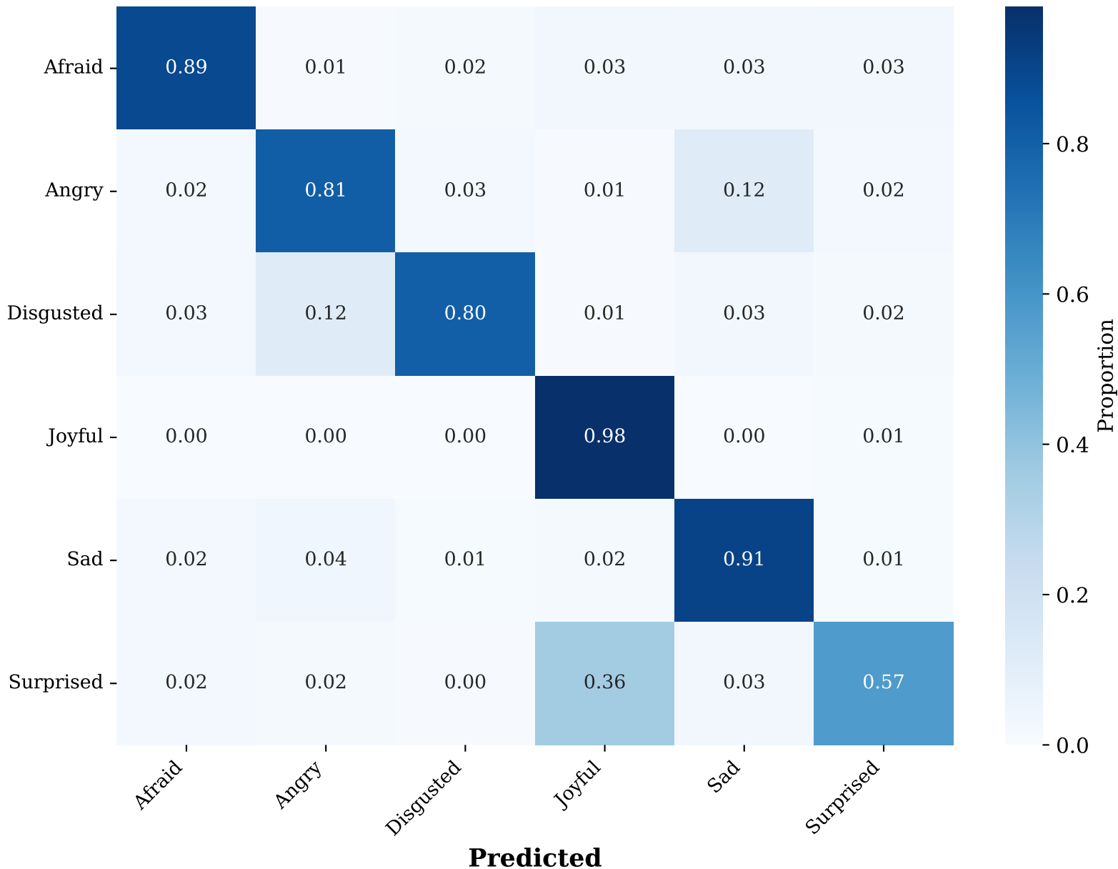
Baseline Confusion Matrix (6-Emotion) - Percentages
