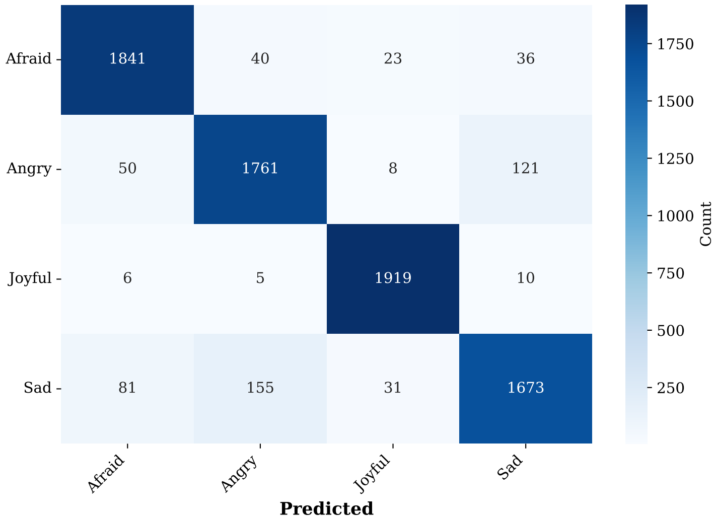
Theory-Guided Confusion Matrix (4-Emotion)
