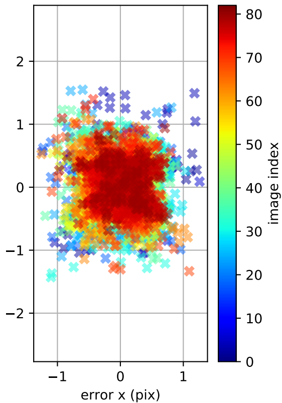
cam3: reprojection errors
