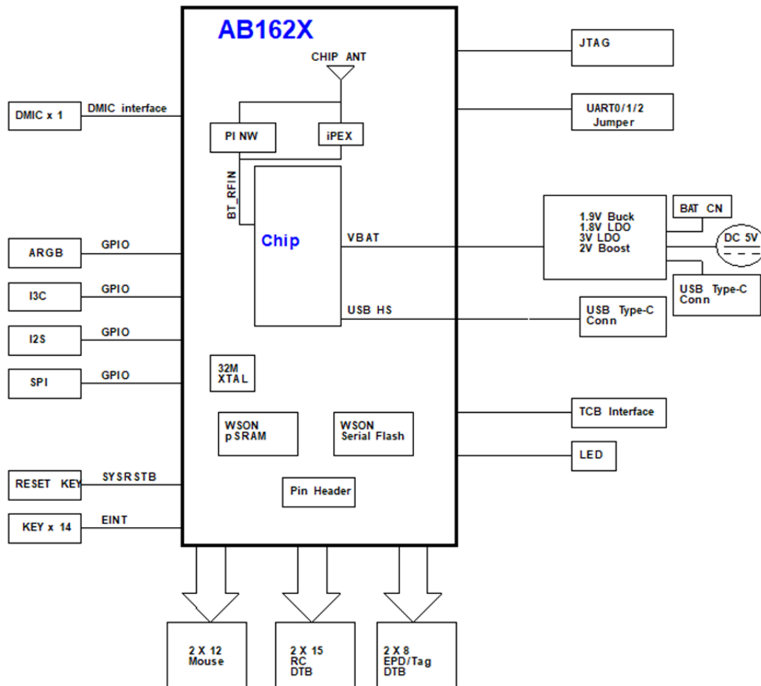
Figure 1. Block Diagram of the AB162x Series EVK
