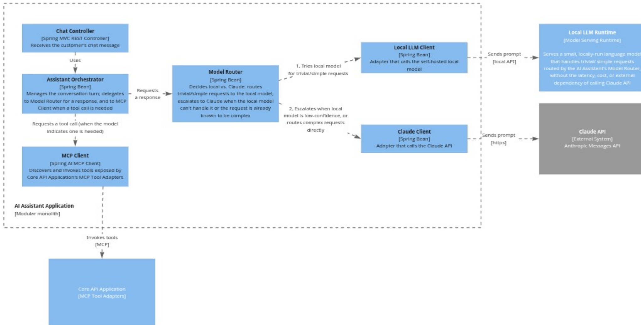
Component Diagram for Roam & Frame - AI Assistant
