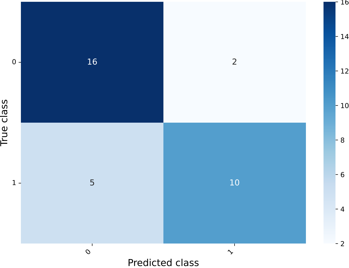
Confusion Matrix
