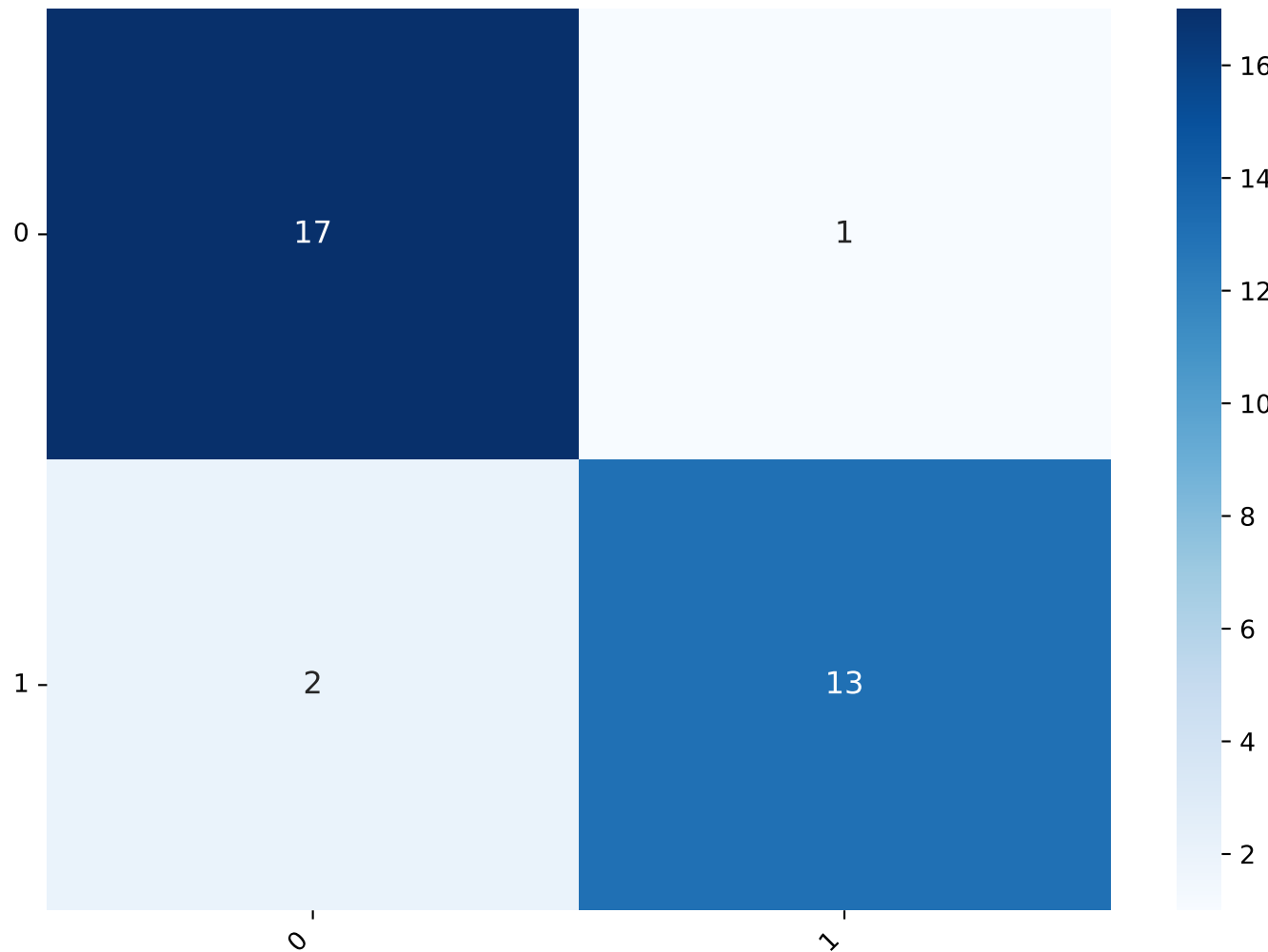
Confusion Matrix
