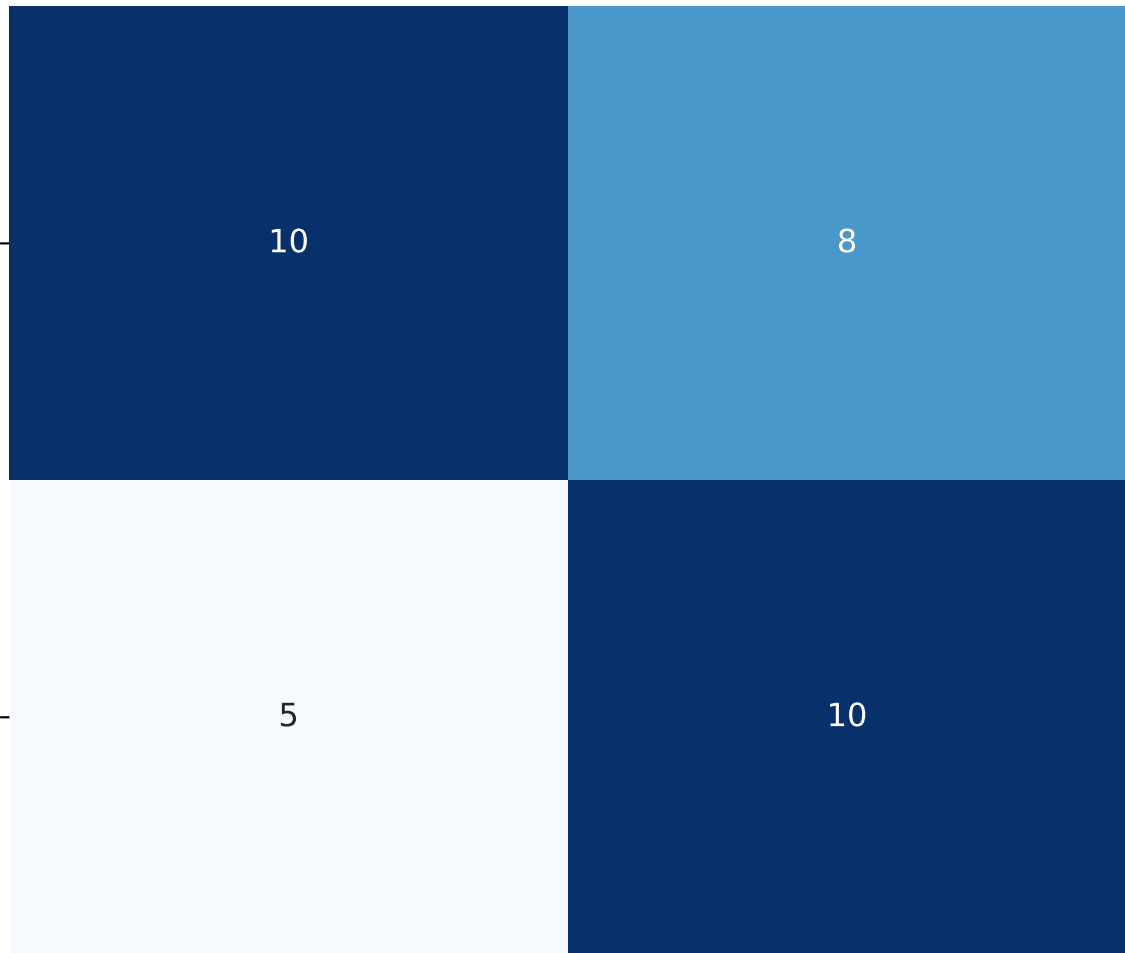
Confusion Matrix
