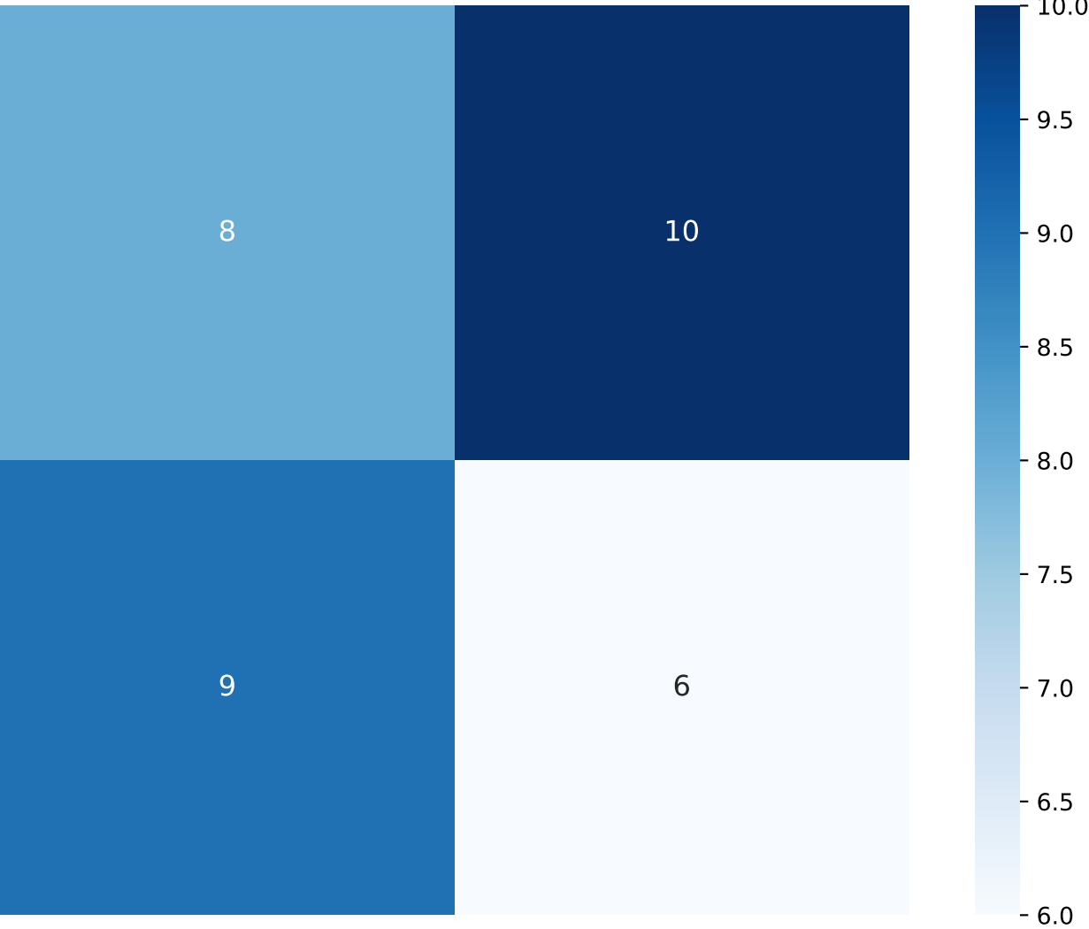
Confusion Matrix
