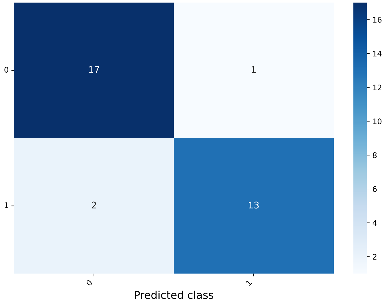
Confusion Matrix
