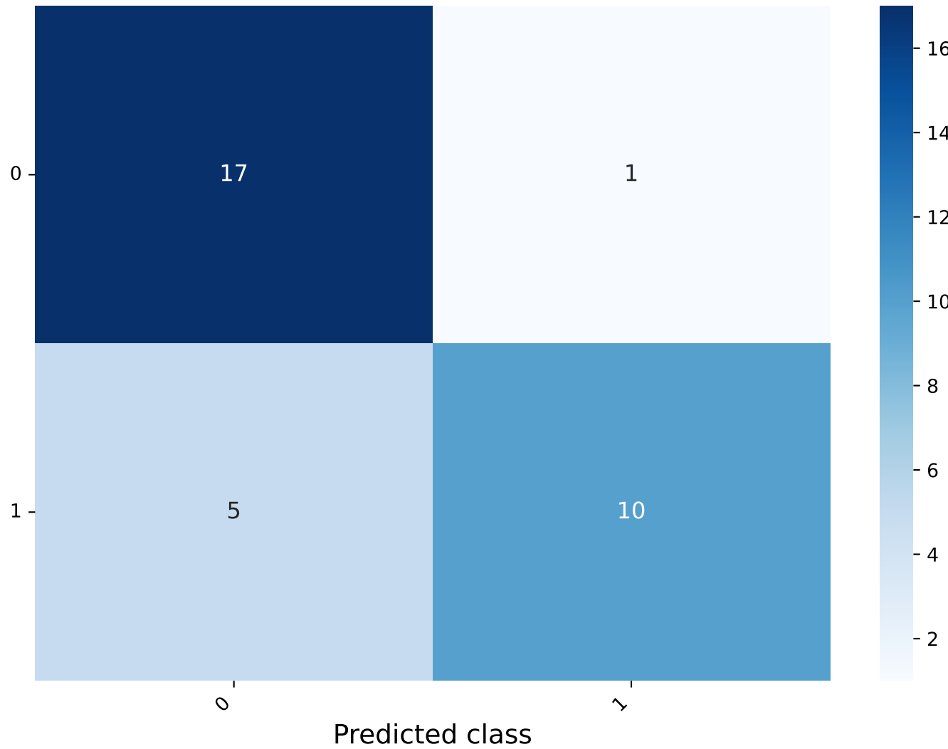
Confusion Matrix
