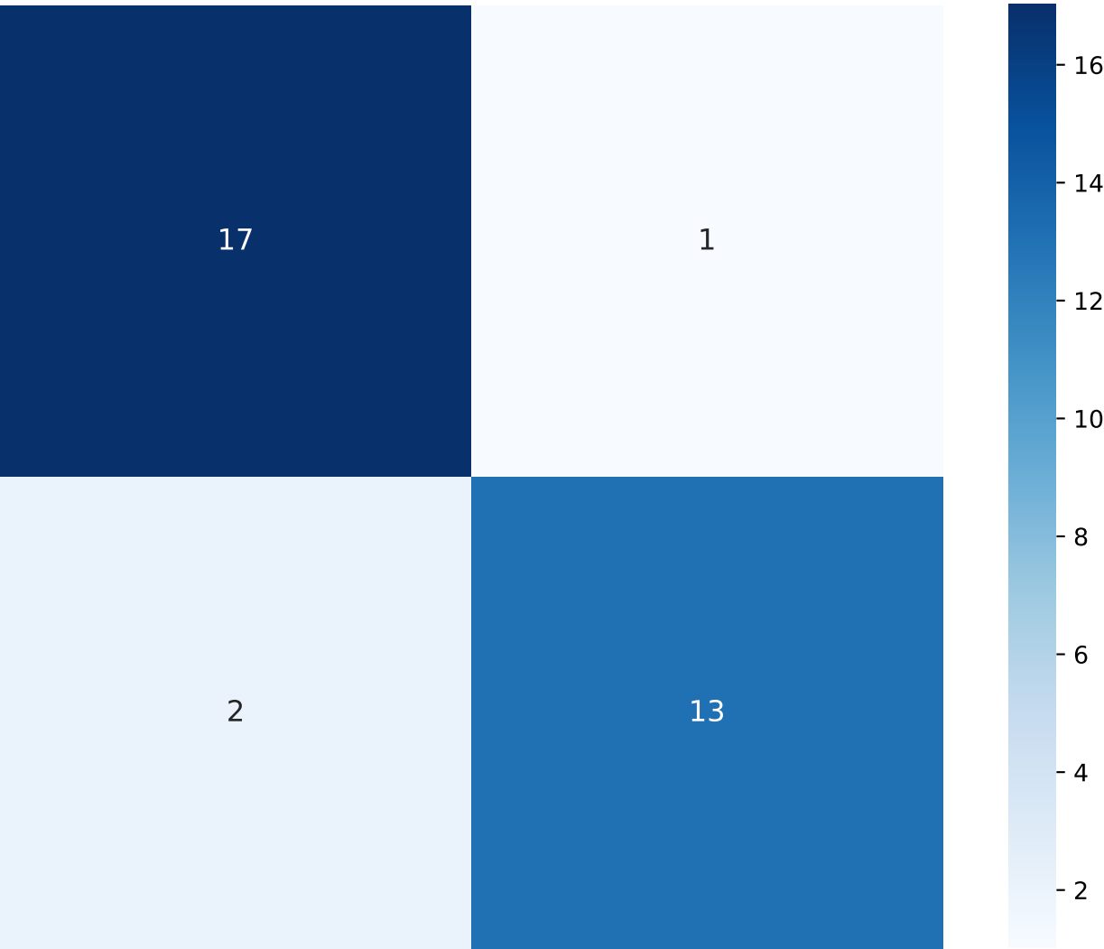
Confusion Matrix
