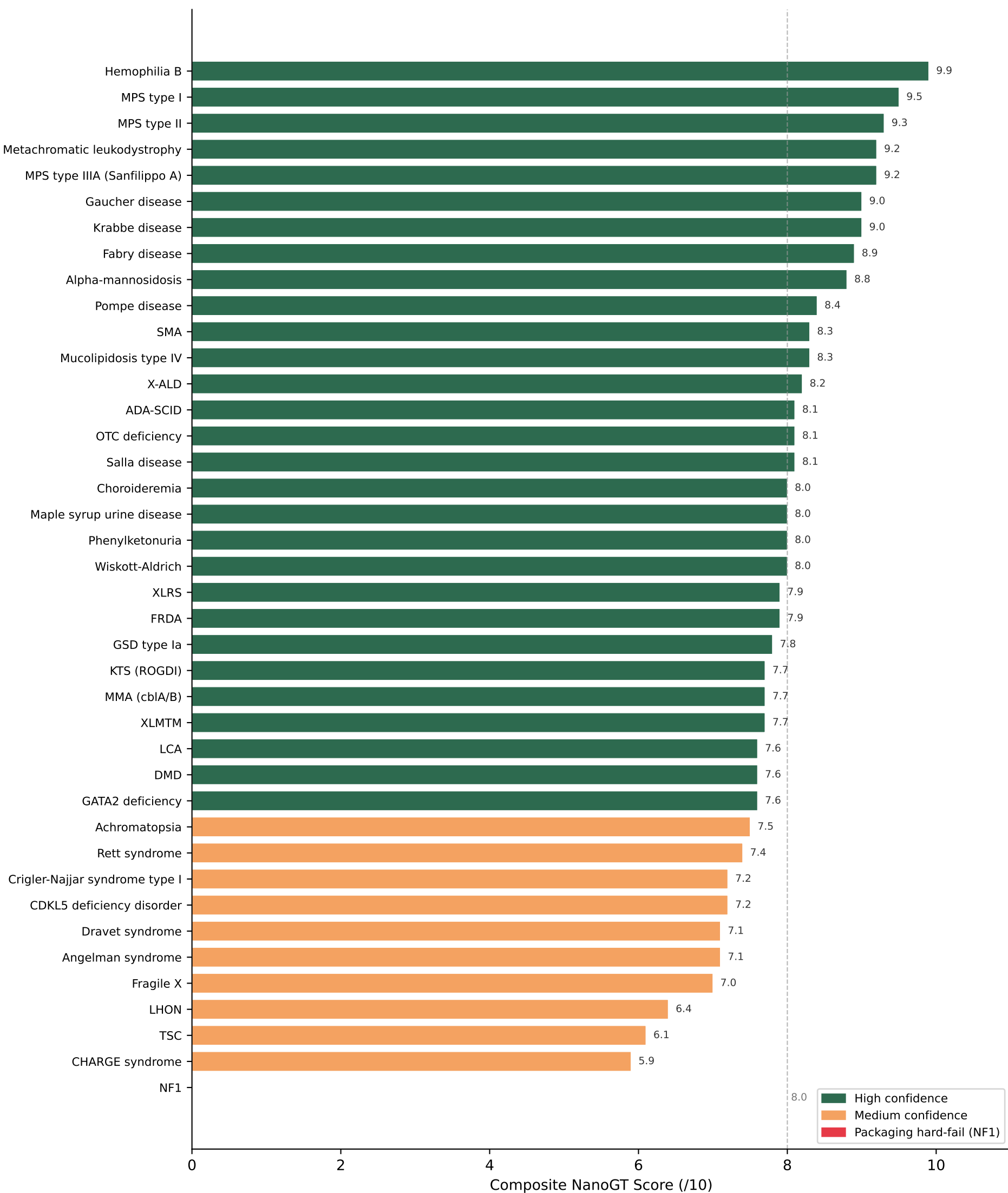
Figure 1: NanoGT Composite Scores — 40-Disease Cohort
