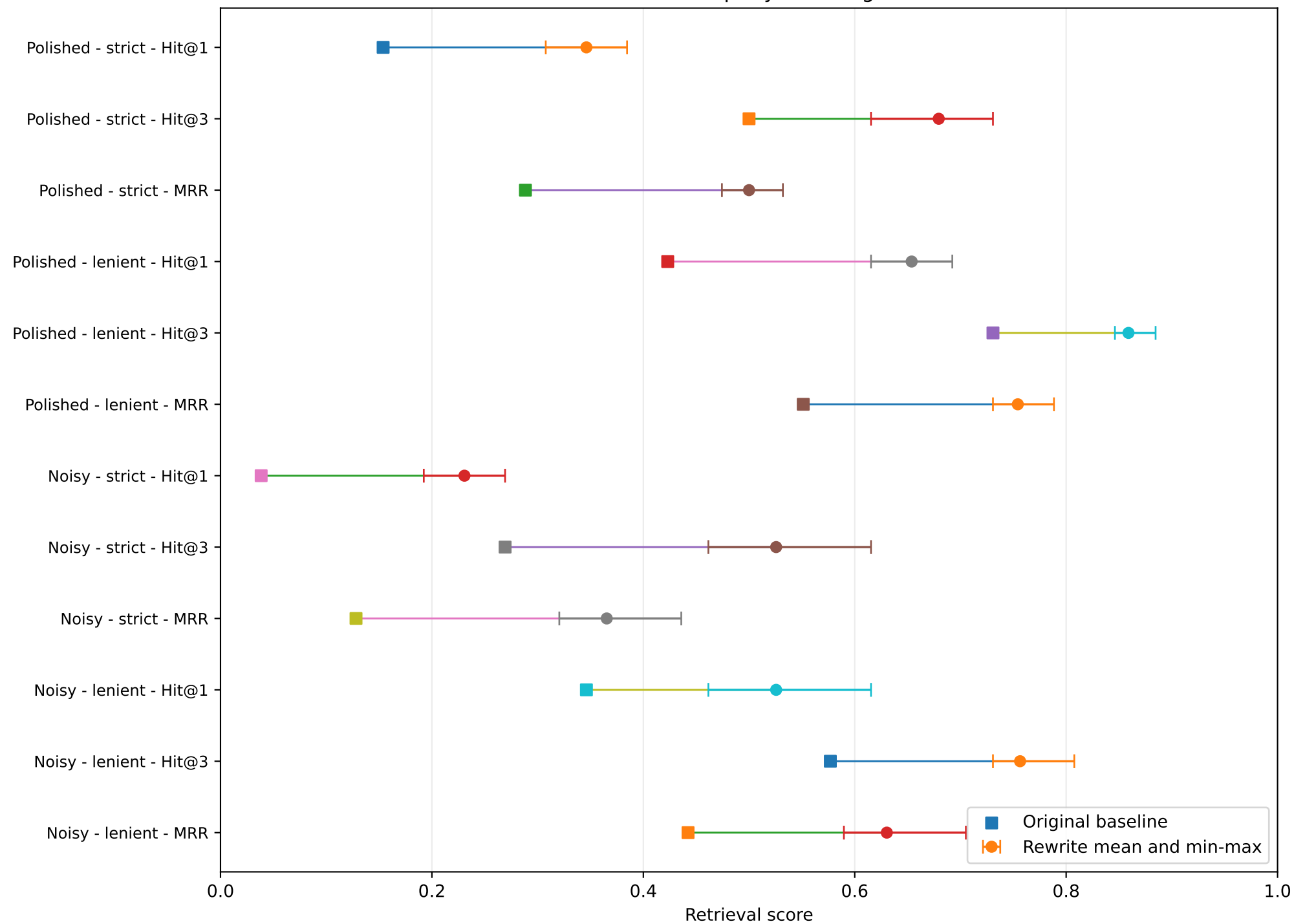
Effect of query rewriting
