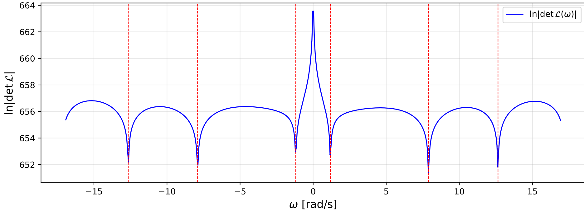
Global SWMHD determinant scan (m=1)
