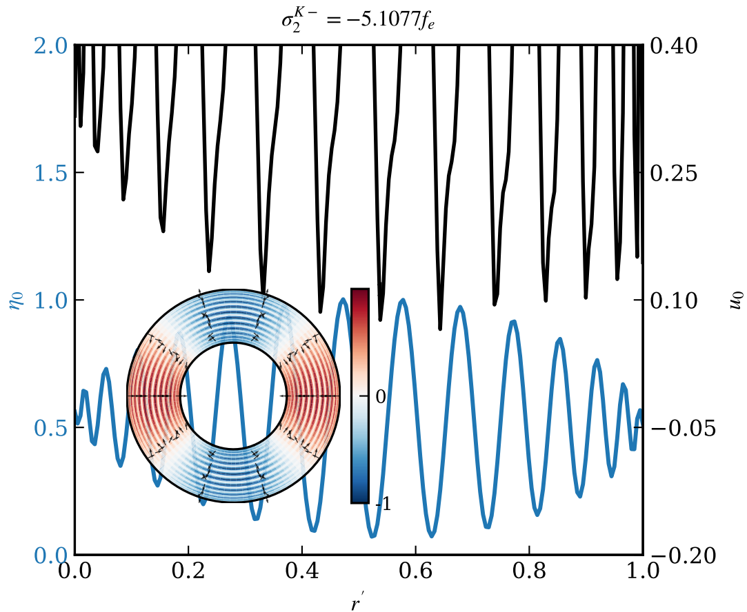
(a) Counter-rotating Kelvin waves.
