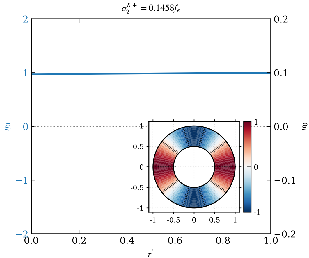
(b) Co-rotating Kelvin waves.
