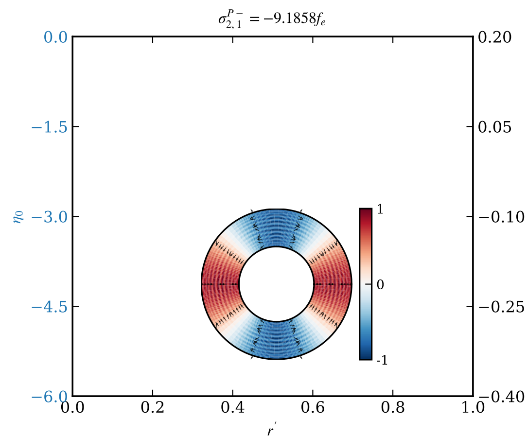
(a) Counter-rotating Poincaré waves.
