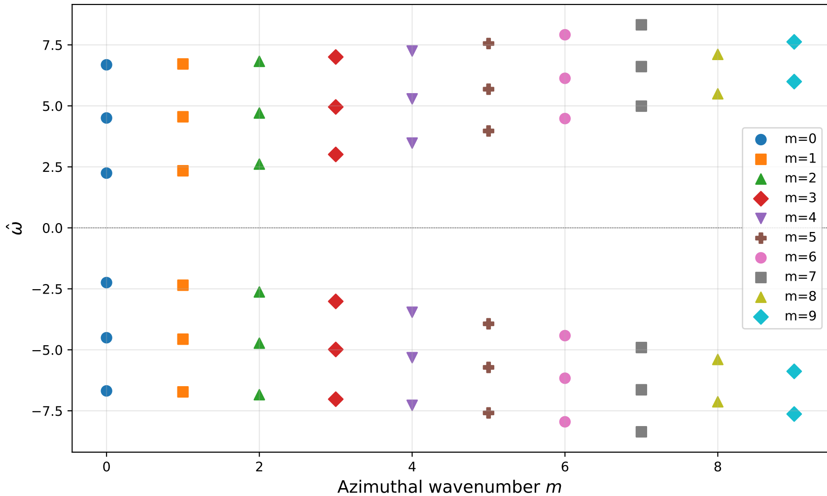
Global SWMHD dispersion relation (dimensionless, \hat{\omega} vs m )
