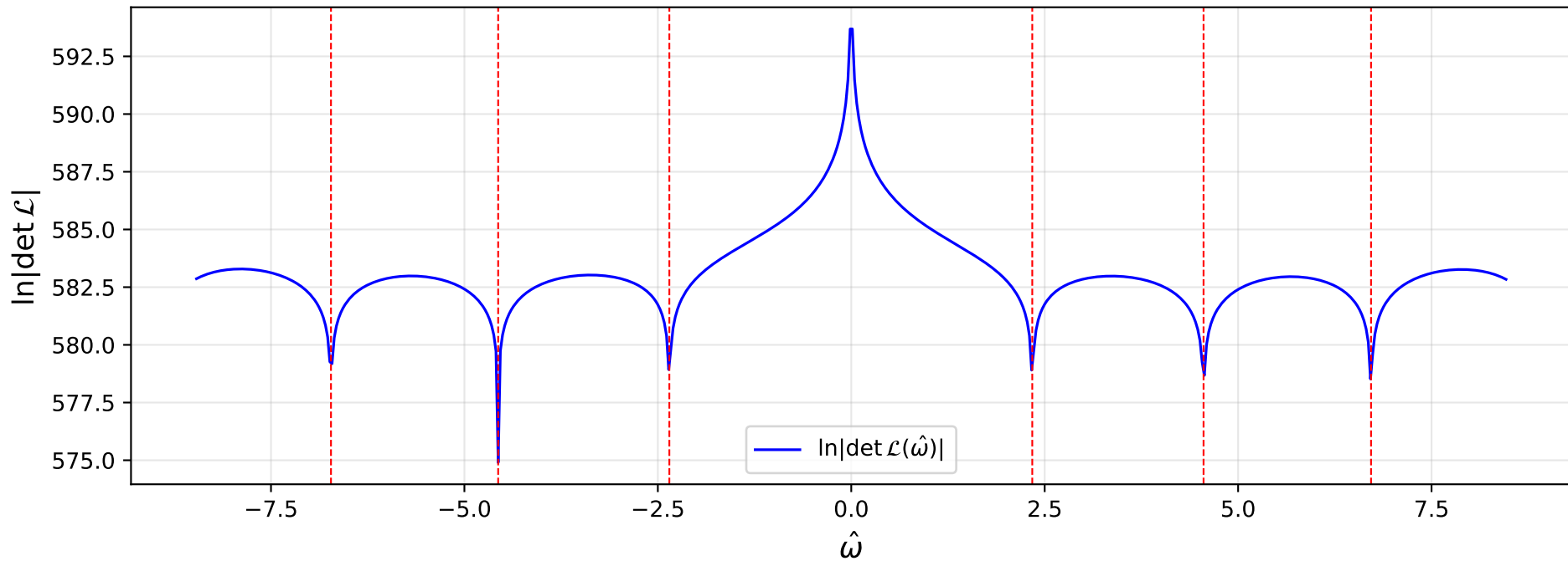
Global SWMHD determinant scan (dimensionless, m=1 )
