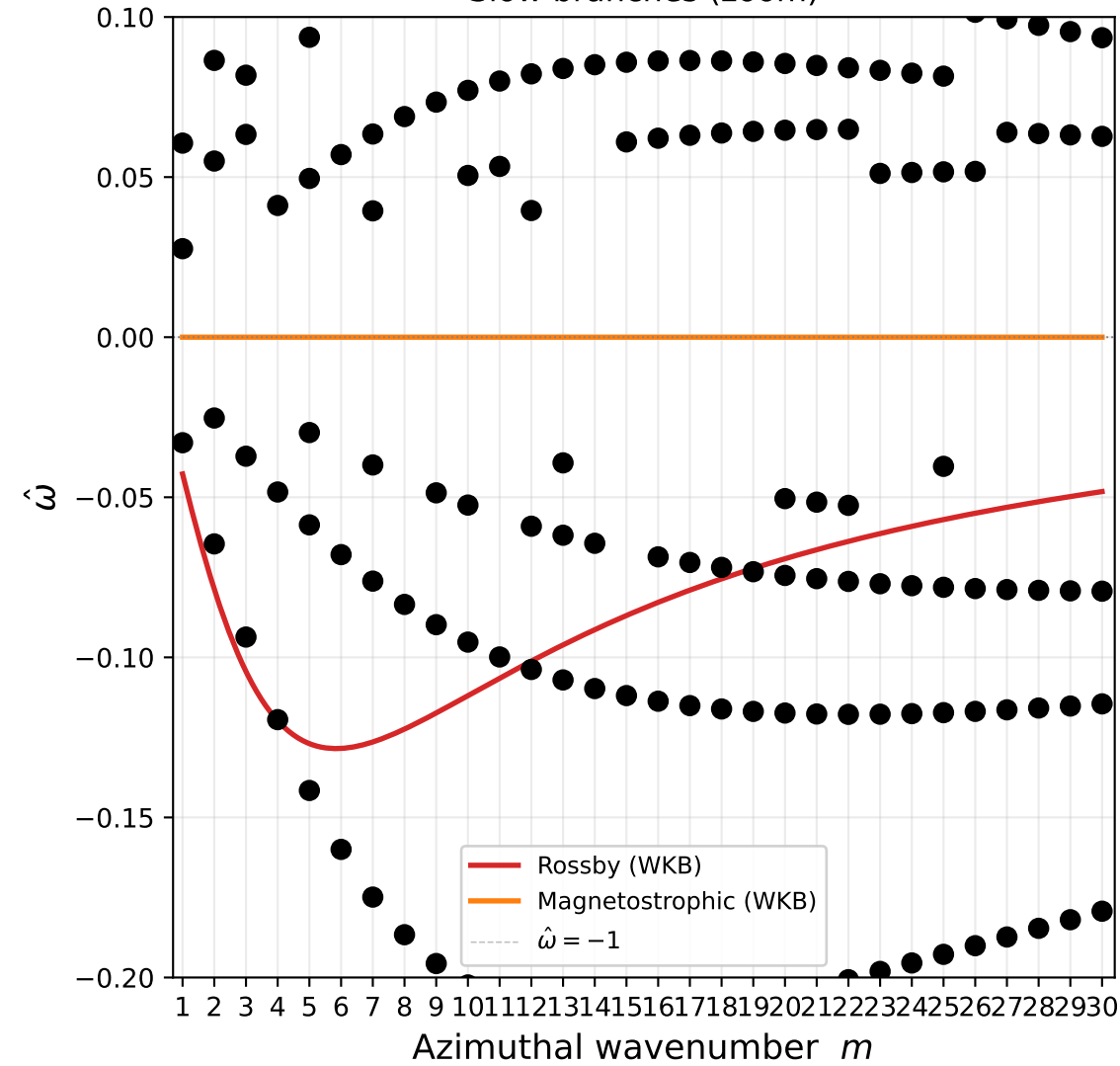
Slow branches (zoom)
