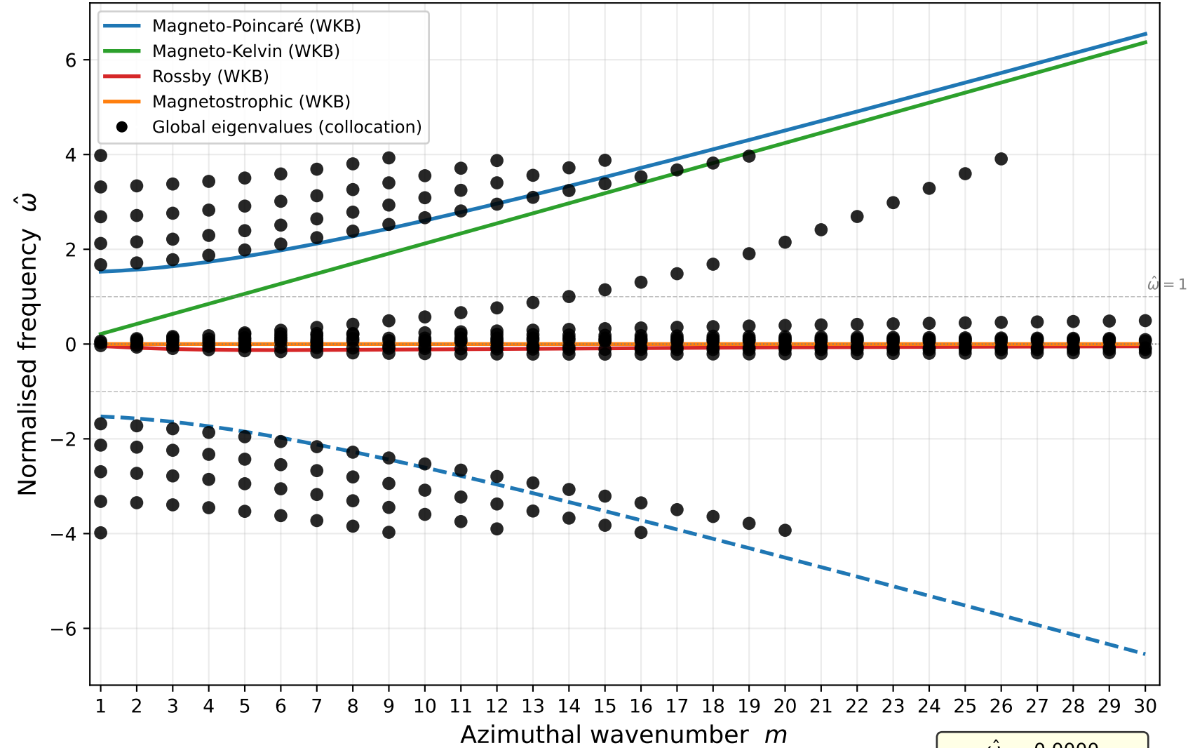
SWMHD global dispersion relation ( \hat{\omega} vs m , dimensionless)
