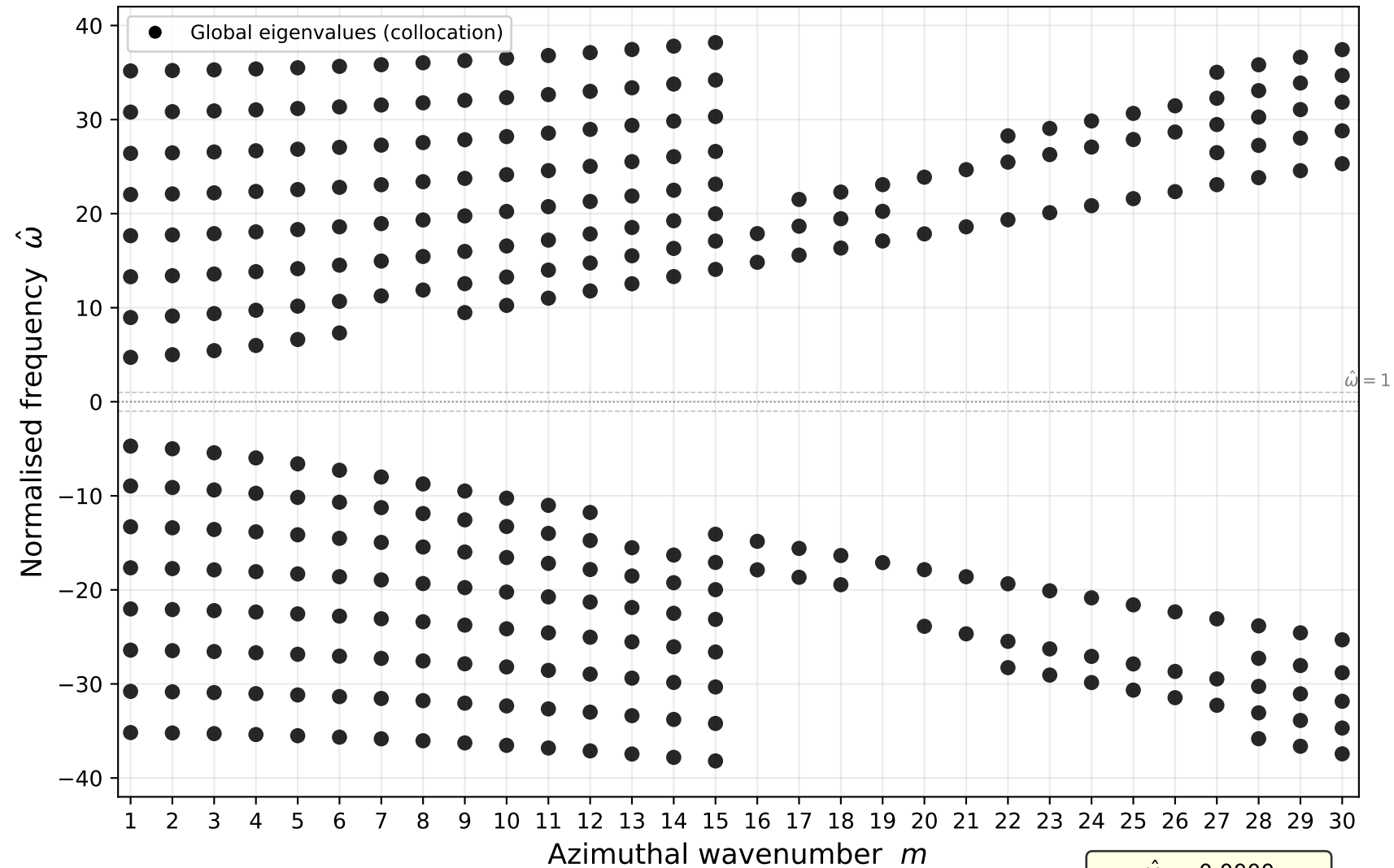
SWMHD global dispersion relation (\hat{\omega} \text{ vs } m, \text{ dimensionless})
