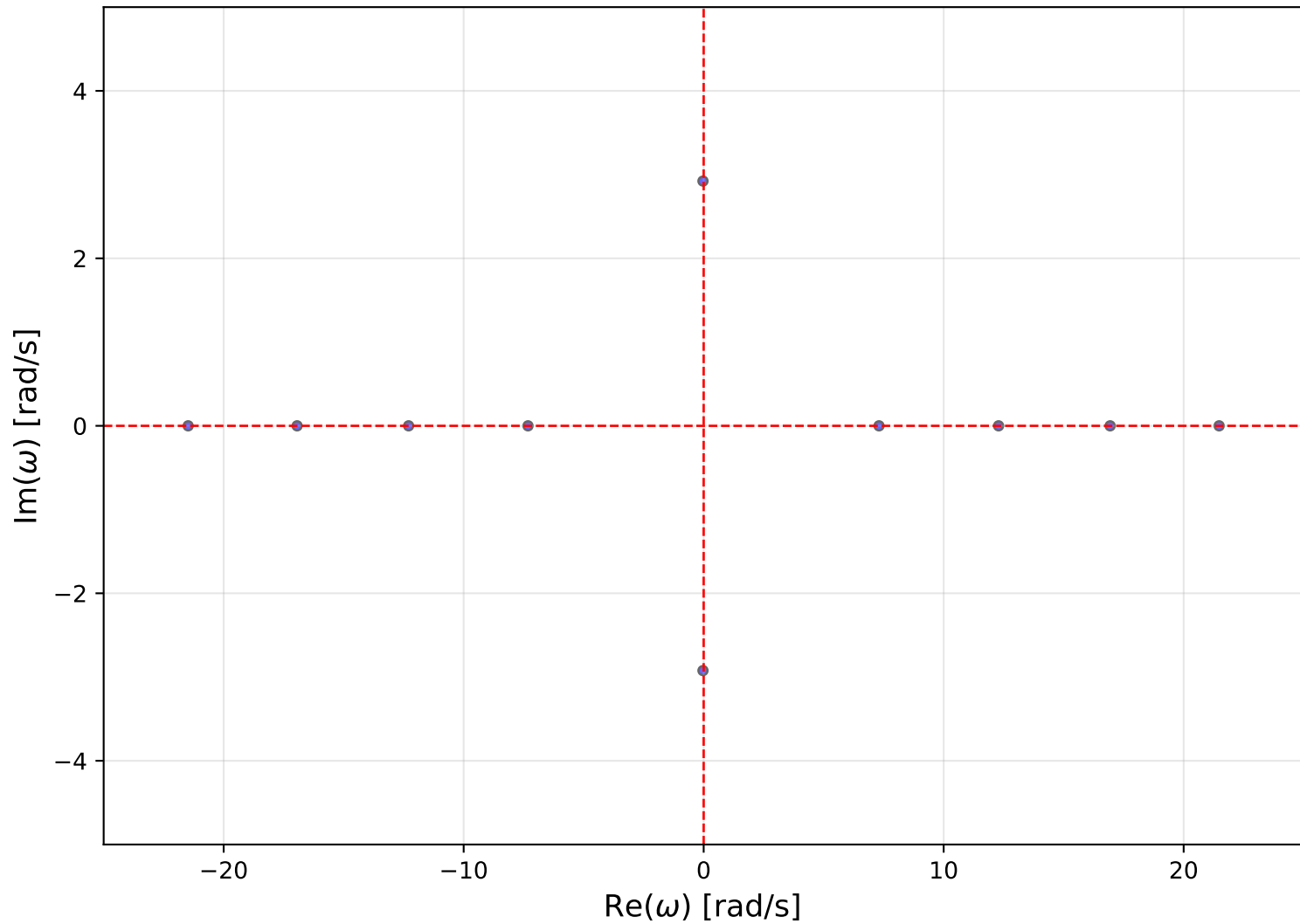
Global SWMHD Spectrum via 5N x 5N GEVP (m=1, C=0.5)
