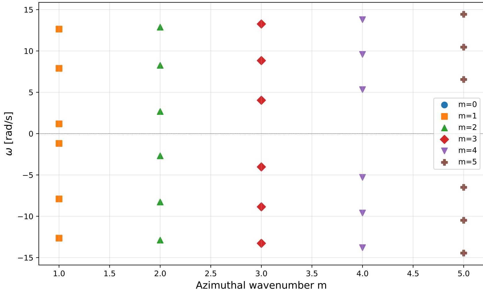
Global SWMHD dispersion relation (eigenfrequencies vs m )
