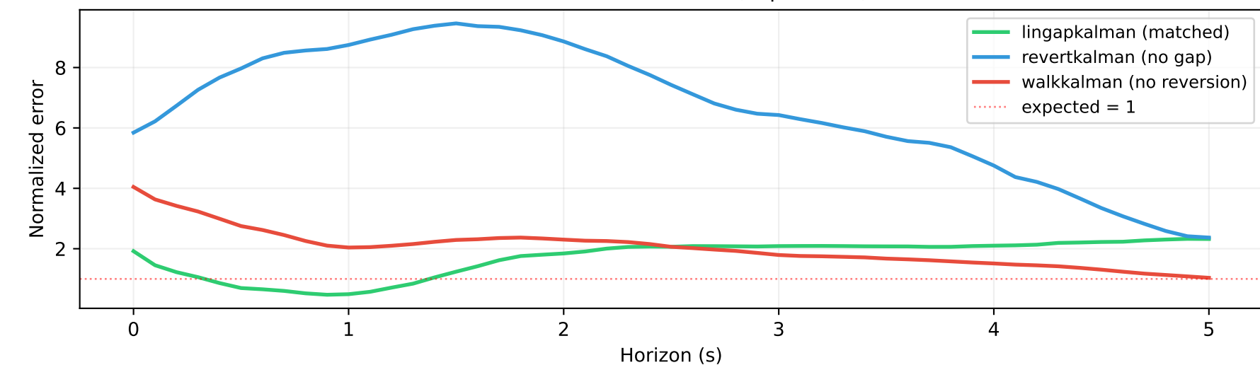
Normalized rollout error (expect \approx 1 )
