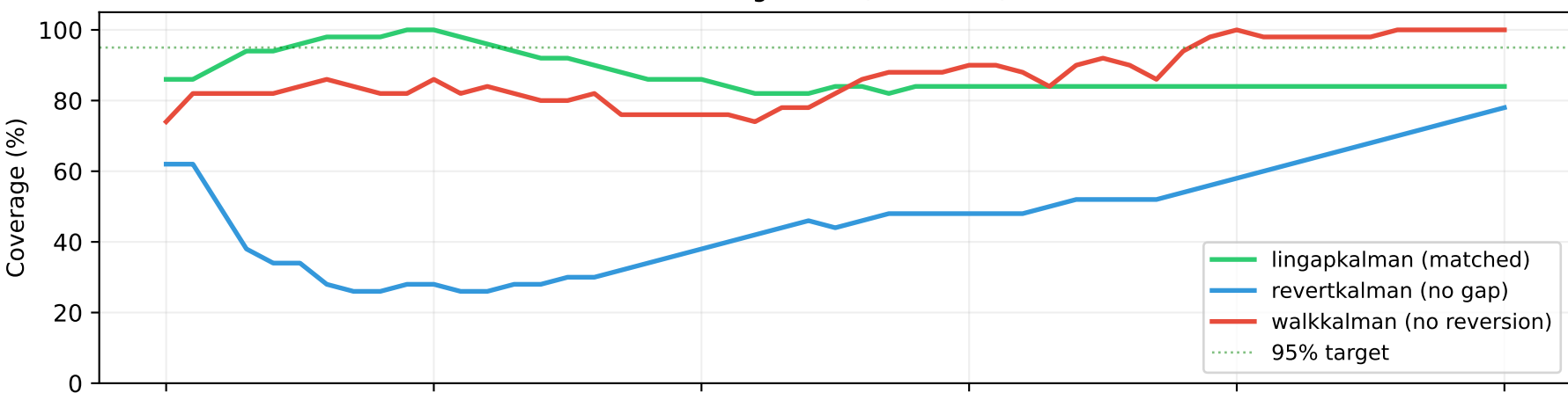
Coverage rate ( \pm 2\sigma band)
