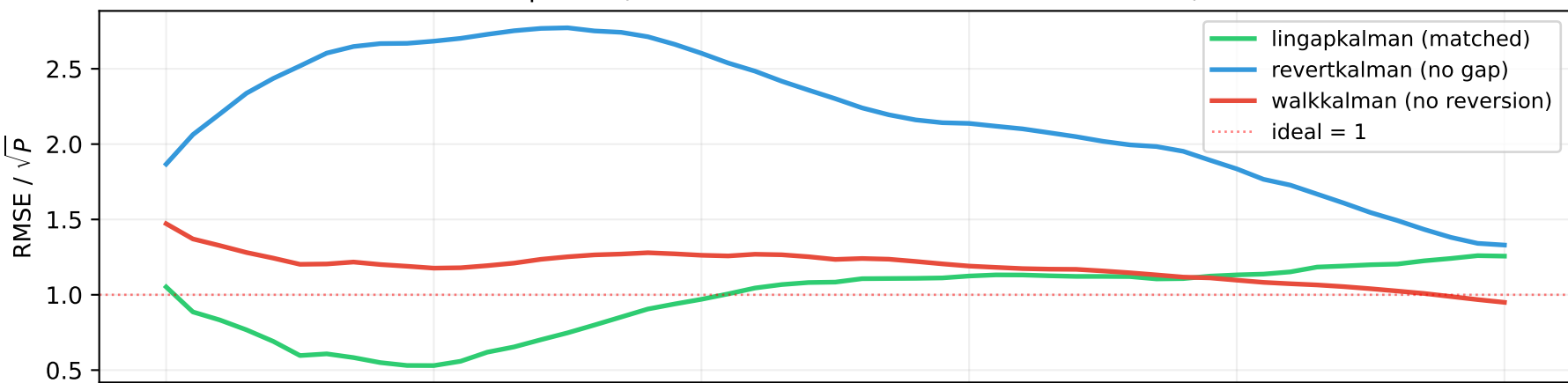
Sharpness ( < 1 = underconfident, > 1 = overconfident)
