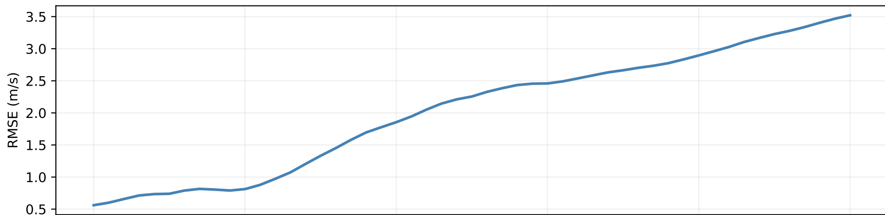
Rollout RMSE vs horizon
