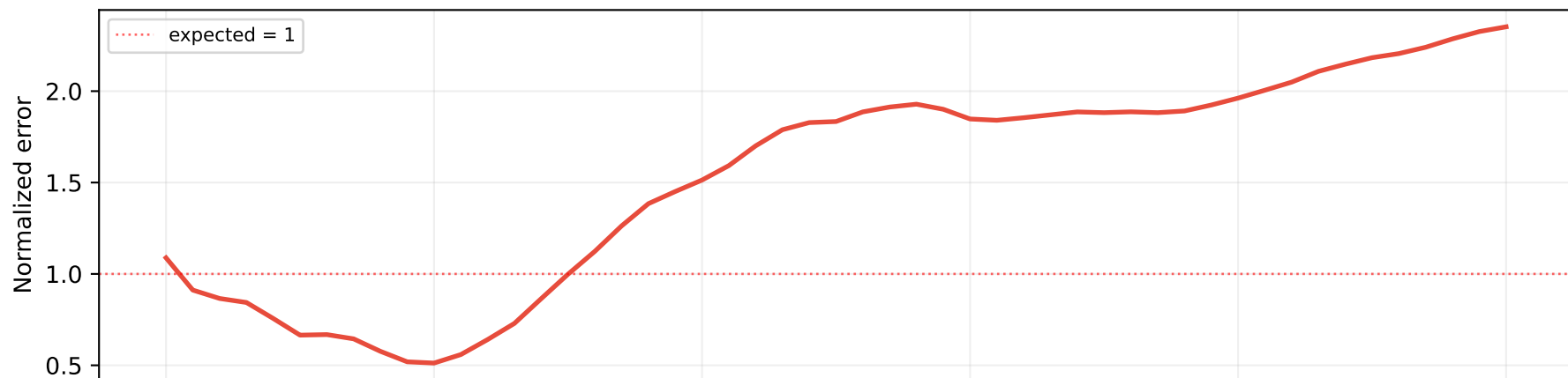
Normalized rollout error (expect \approx 1 if P calibrated)
