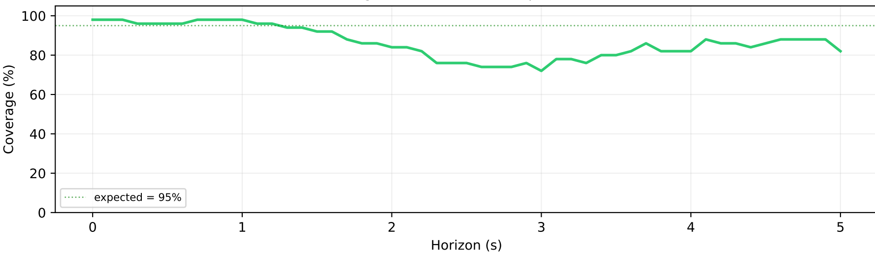
Coverage rate ( \pm 2\sigma band, expect \approx 95\% )
