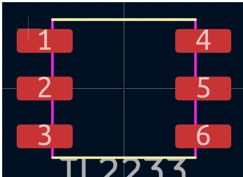
TL2233 Push-Button Switch
