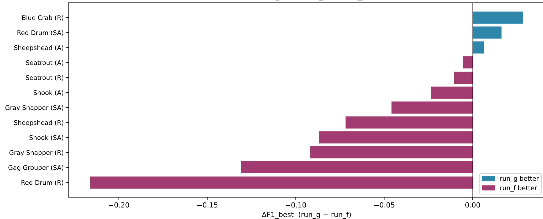
Per-species \Delta F1_{\text{best}} : run_g vs run_f (8 folds)
