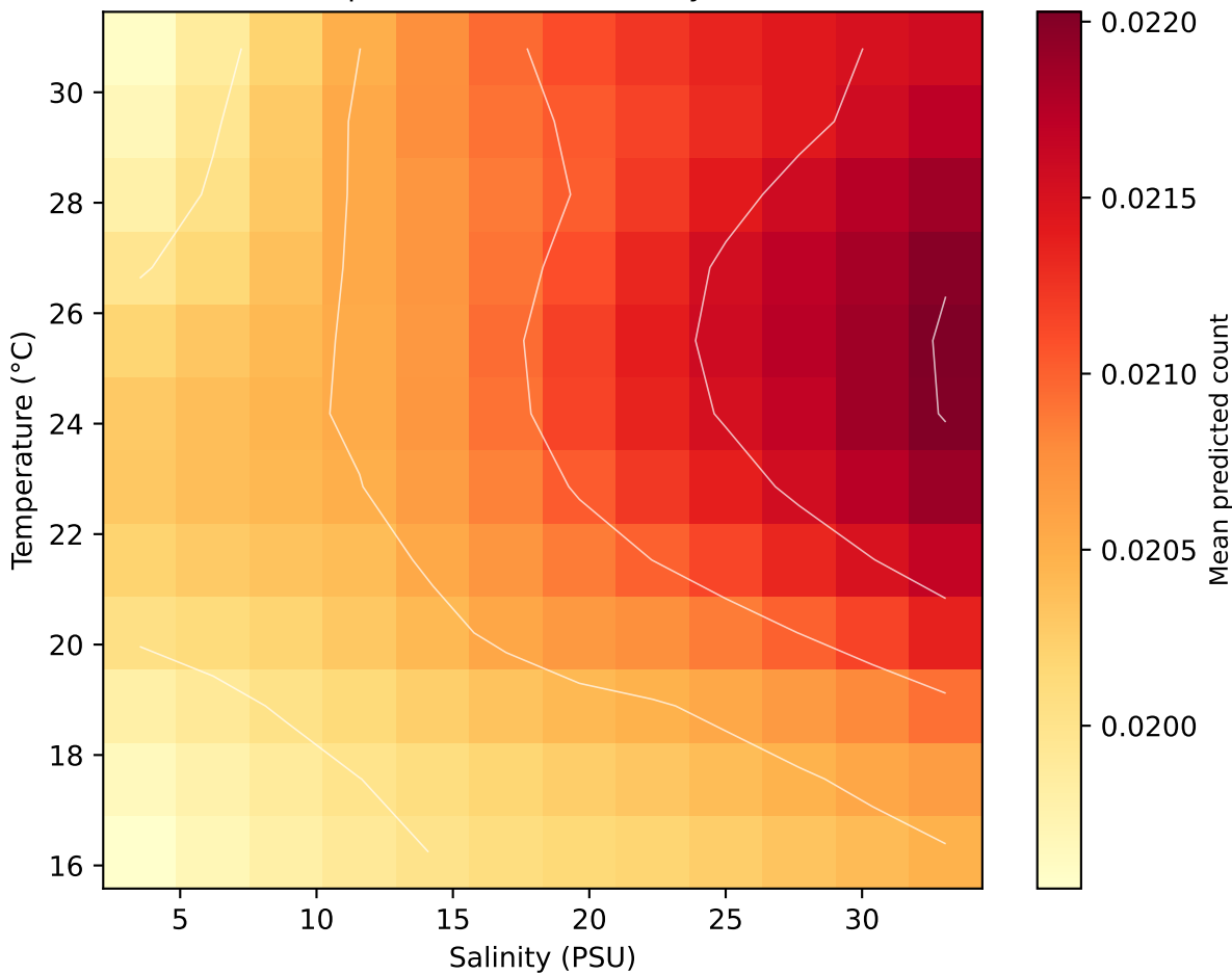
2-D PDP: Red Drum (Recruit) (Temperature (°C) × Salinity (PSU))
