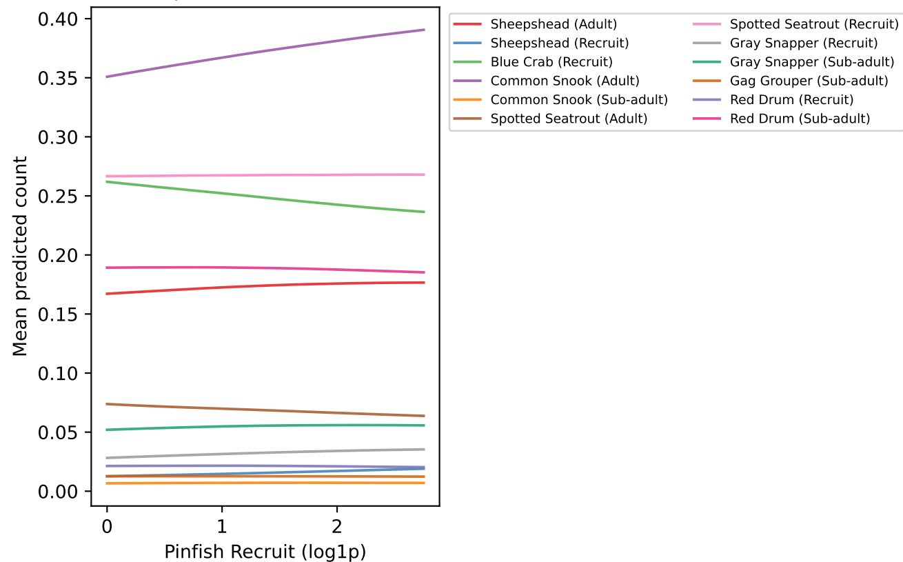
Partial Dependence on Pinfish Recruit
