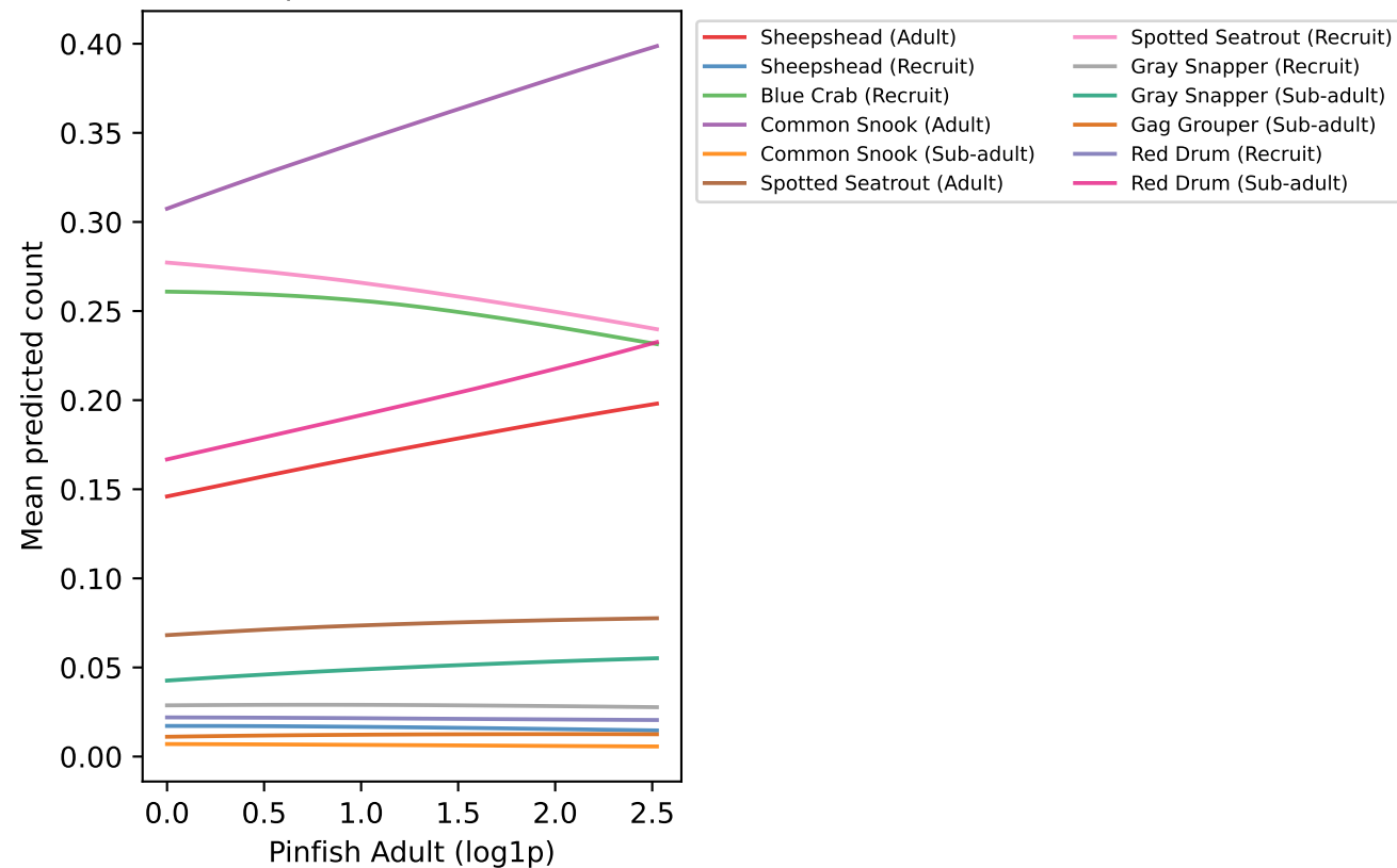
Partial Dependence on Pinfish Adult
