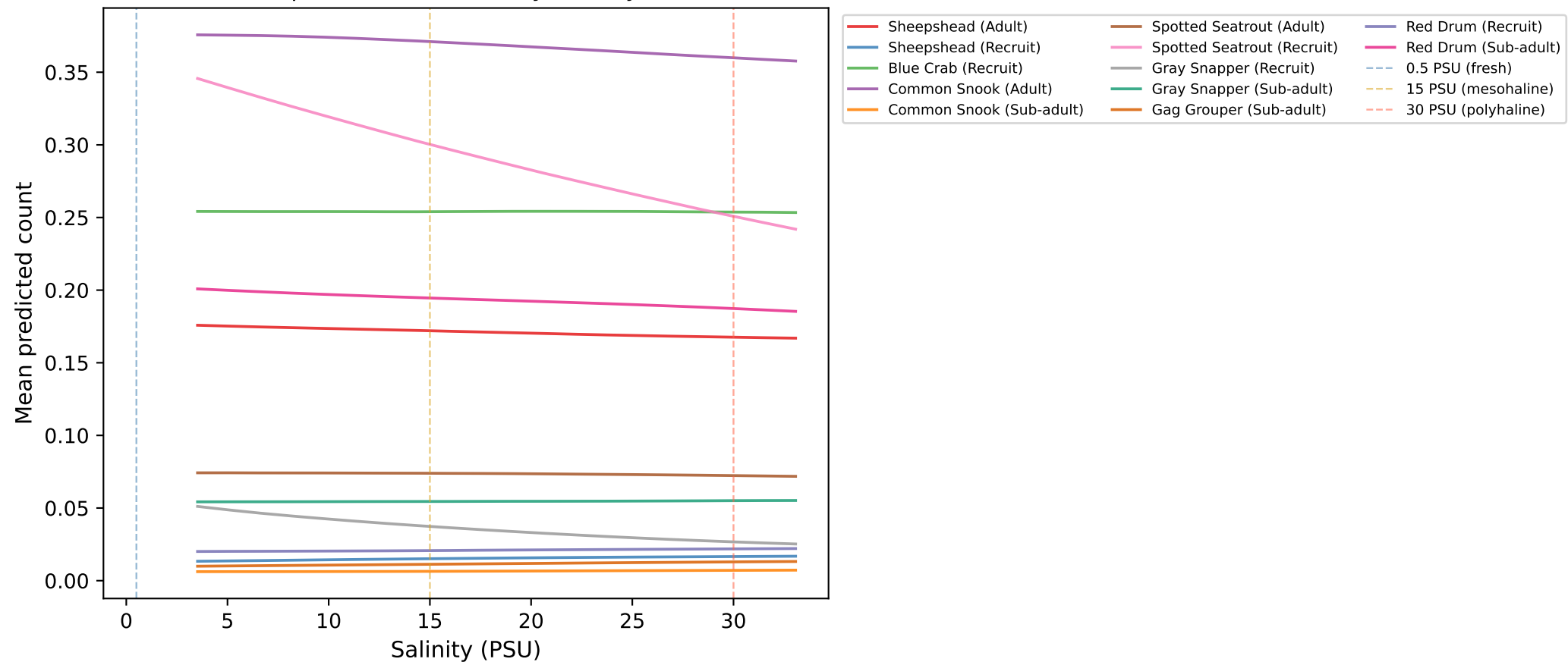
Partial Dependence on Salinity (test year 2024)
