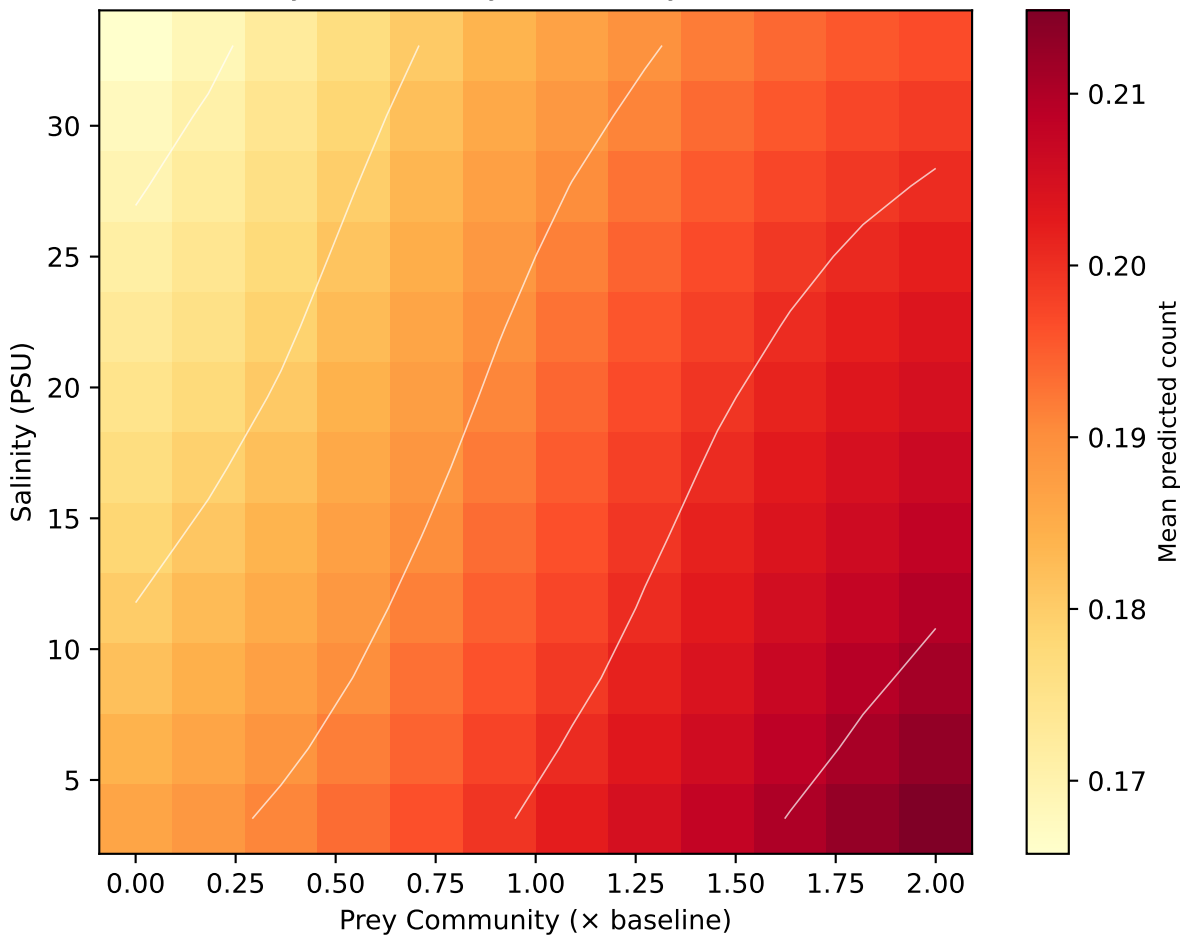
2-D PDP: Red Drum (Sub-adult) (Salinity (PSU) \times Prey Community ( \times baseline))
