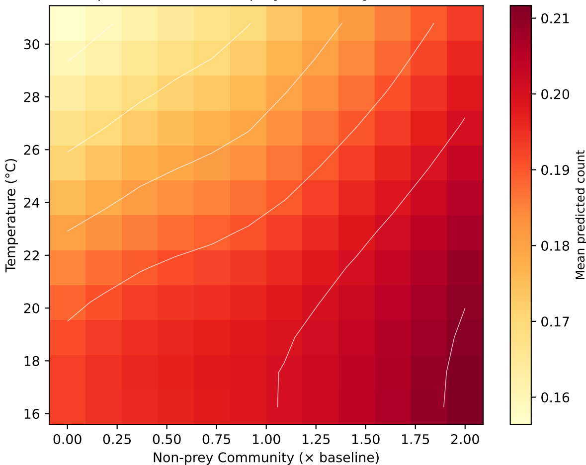
2-D PDP: Red Drum (Sub-adult) (Temperature ( ^{\circ}\text{C} ) \times Non-prey Community ( \times baseline))
