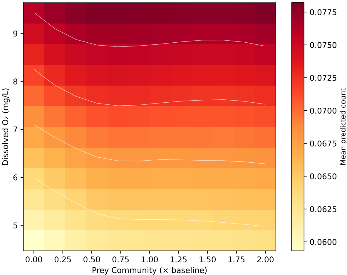
2-D PDP: Spotted Seatrout (Adult) (Dissolved O 2 (mg/L) × Prey Community (× baseline))
