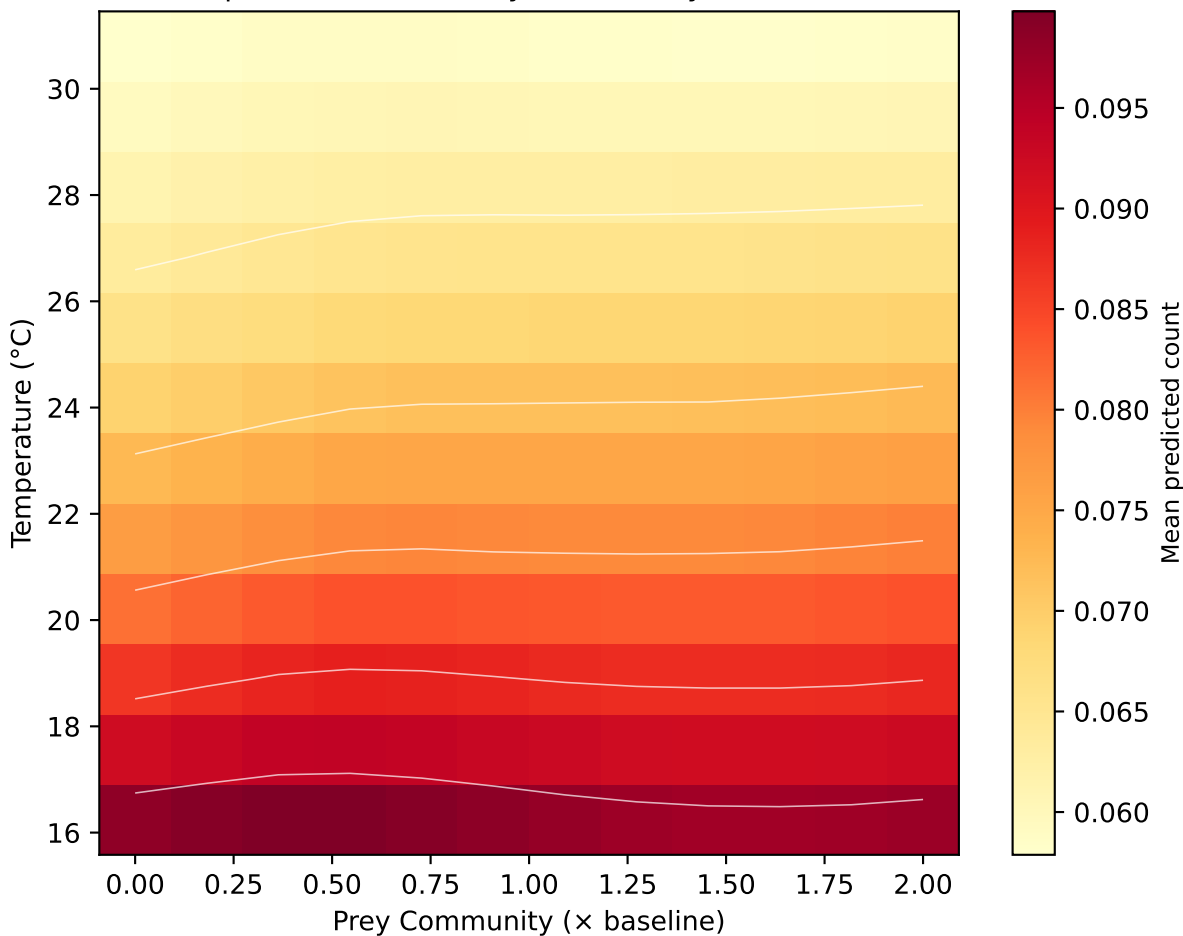
2-D PDP: Spotted Seatrout (Adult) (Temperature (°C) × Prey Community (× baseline))
