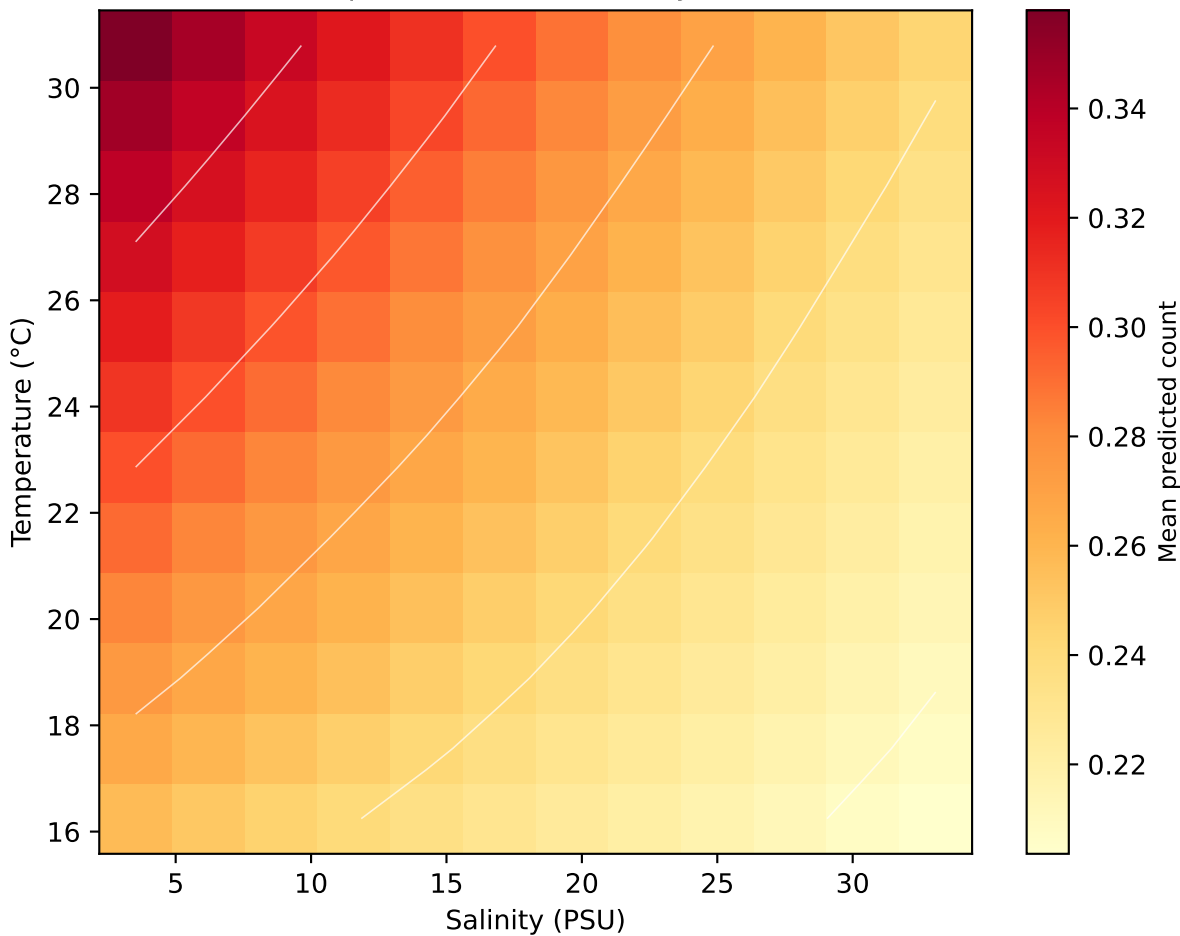
2-D PDP: Spotted Seatrout (Recruit) (Temperature (°C) × Salinity (PSU))
