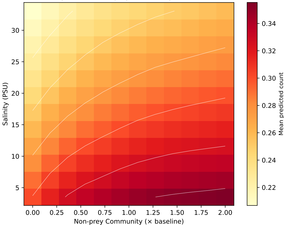
2-D PDP: Spotted Seatrout (Recruit) (Salinity (PSU) \times Non-prey Community ( \times baseline))
