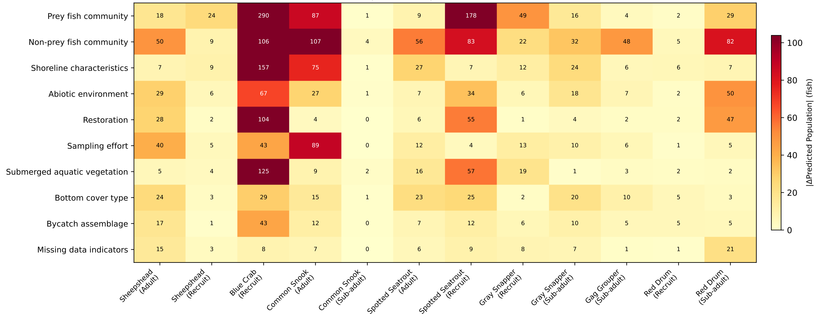
Run H (with restoration) — Feature group effect on predicted population per species
