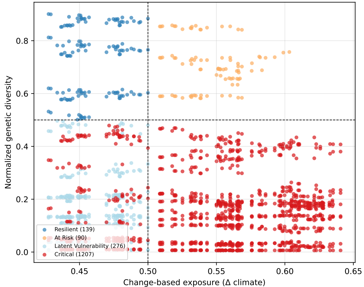
Projected 2100 diversity vs projected climate change
