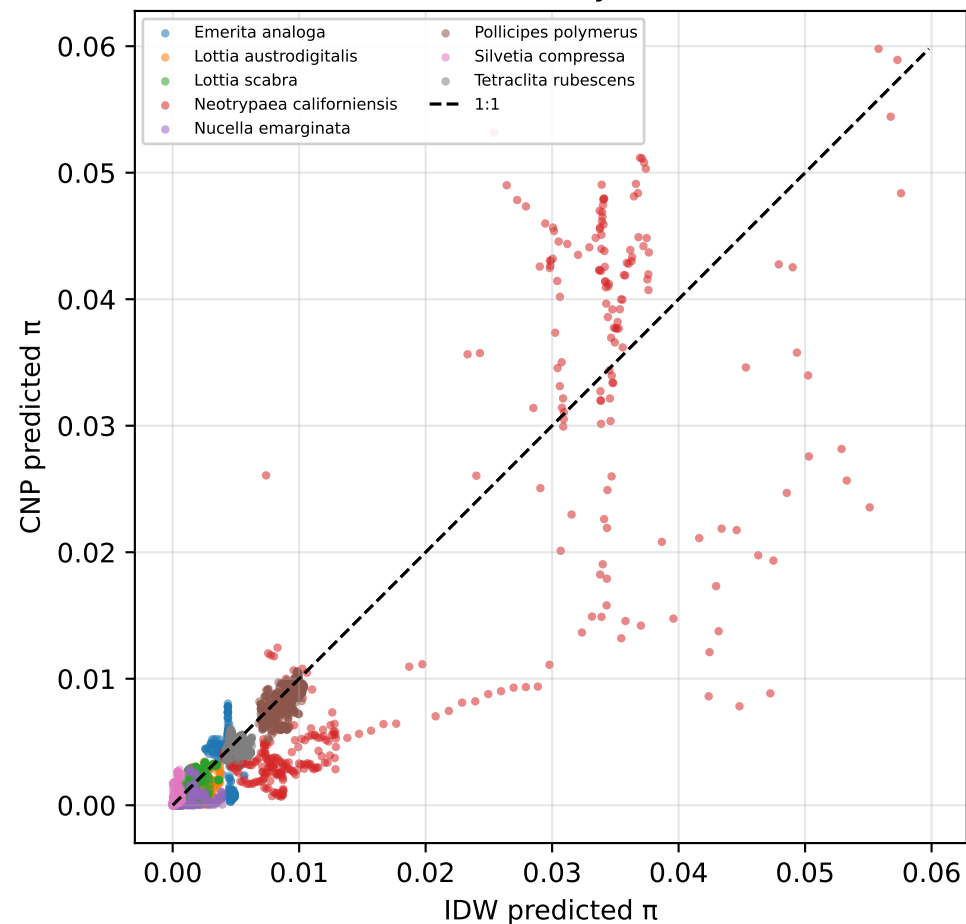
Nucleotide diversity ( \pi ) r=0.89
