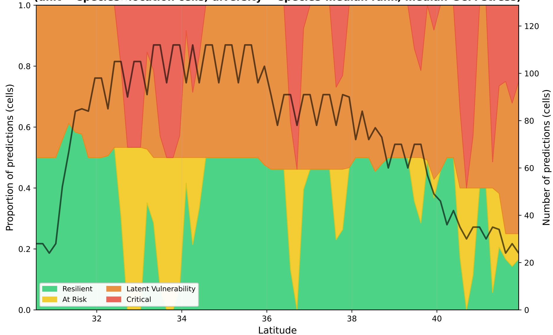
Point-weighted vulnerability composition by latitude (unit = species×location cells; diversity = species-median rank; median-GCM stress)
