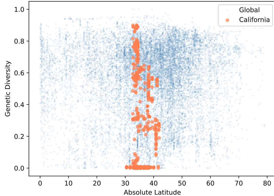
Latitudinal Diversity Gradient
