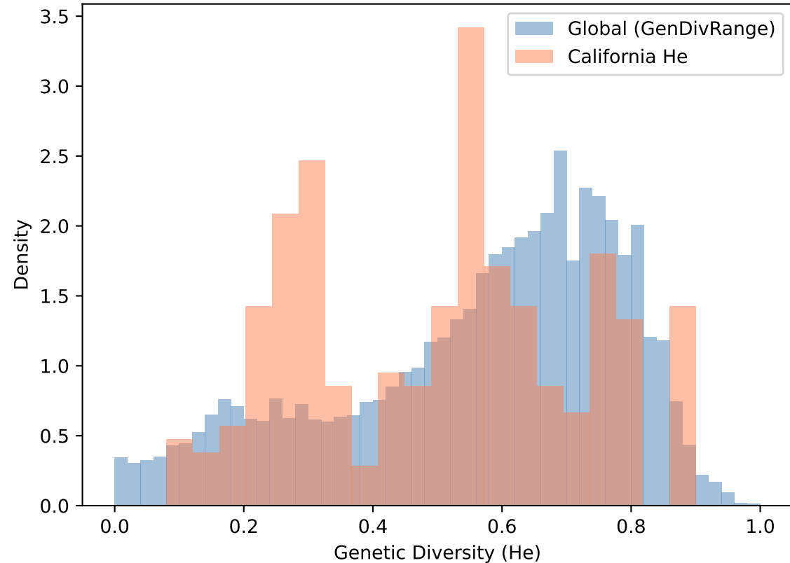
He Distribution: Global vs California
