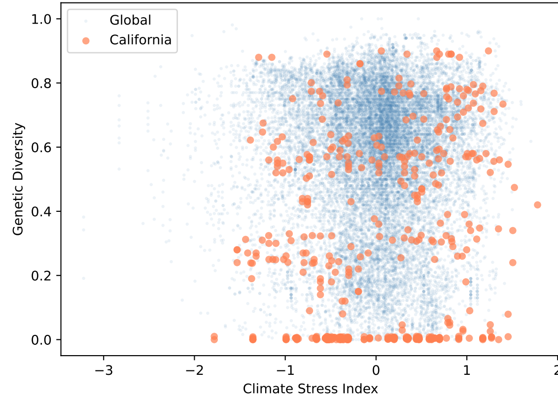
Climate Stress vs Diversity
