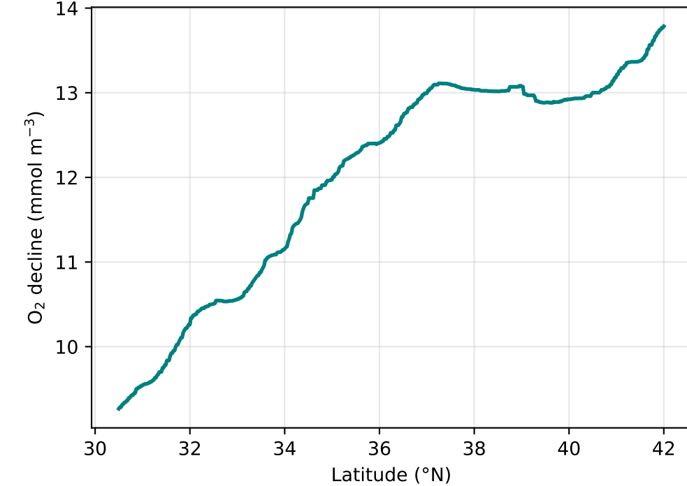
Projected climate CHANGE along the California coast (historical baseline → SSP5-8.5 2081-2100)
