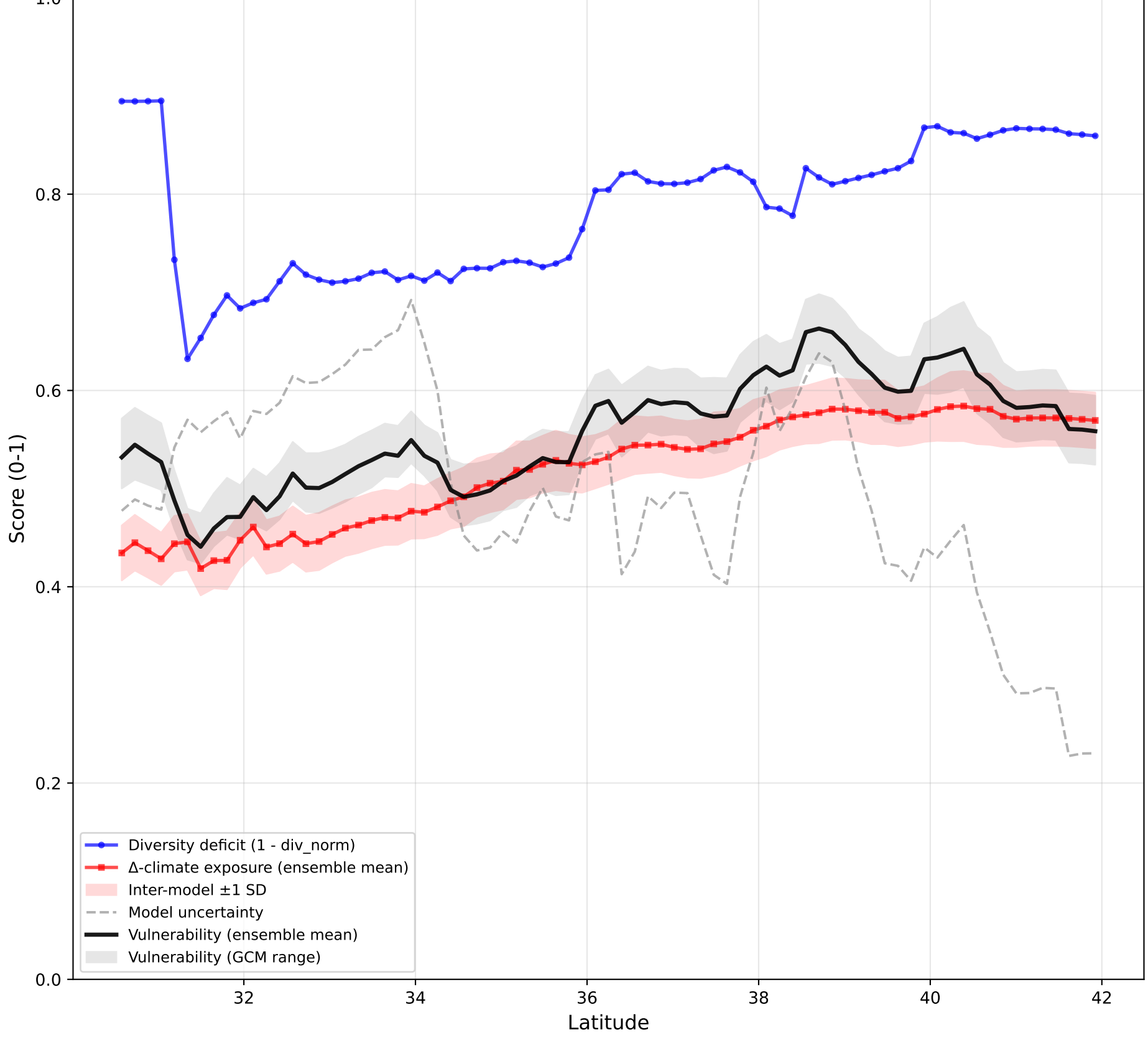
Vulnerability Components (Δ-climate exposure, inter-model uncertainty)
