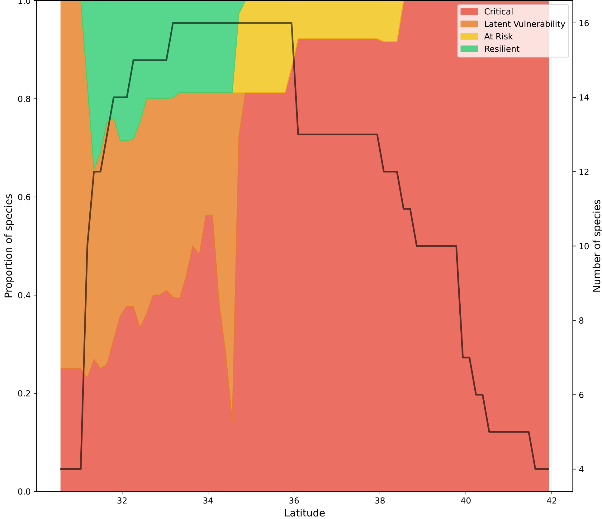
Resilience Class Composition (Δ-climate exposure, ensemble mean)
